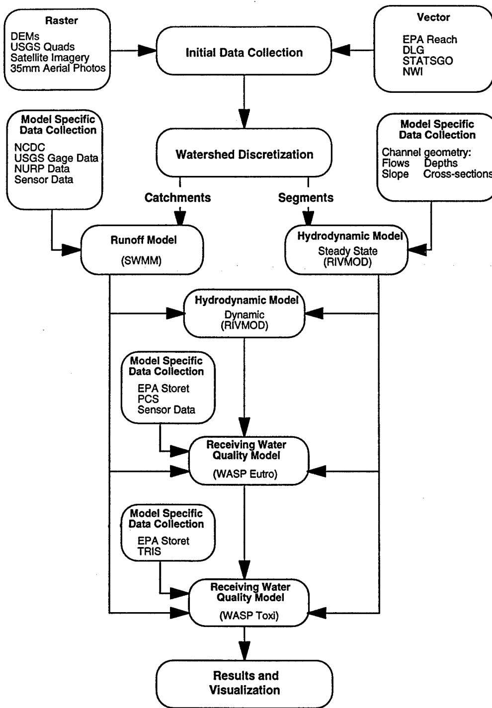
Figure 1. Process Flow
