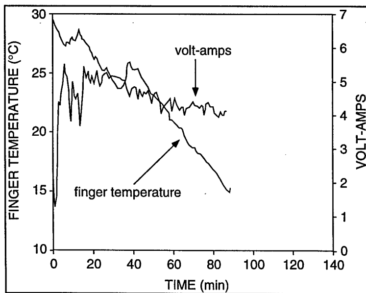
Figure 14. Battery draw and average finger temperatures for Subject 3 wearing ICWG shell over heated liner at -9°C (16°F)
