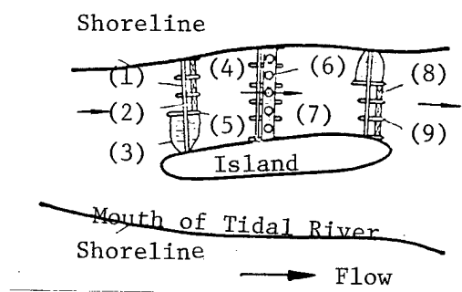
Figure 3. Double Reservoir Unidirectional Tidal Power Station
