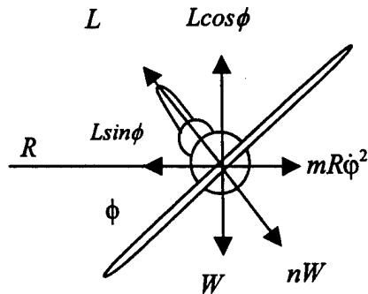
FIGURE 9. STEADY LEVEL BANKED TURN
