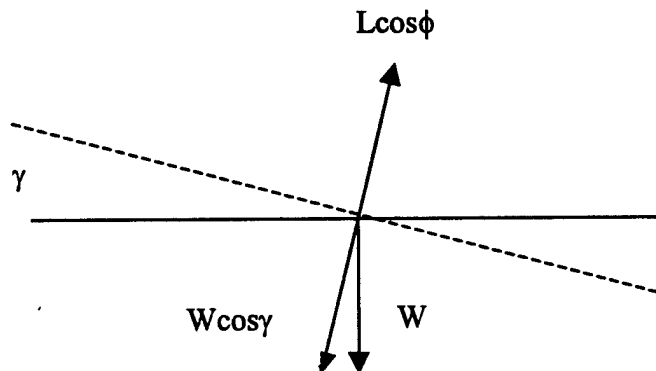
FIGURE A-3. FORCES OF A BANKED TURN DURING CLIMB
