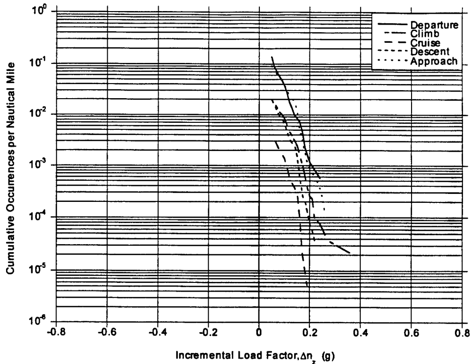
FIGURE 12. CUMULATIVE FREQUENCY OF MANEUVER ACCELERATIONS FAA/NASA CRITERIA
