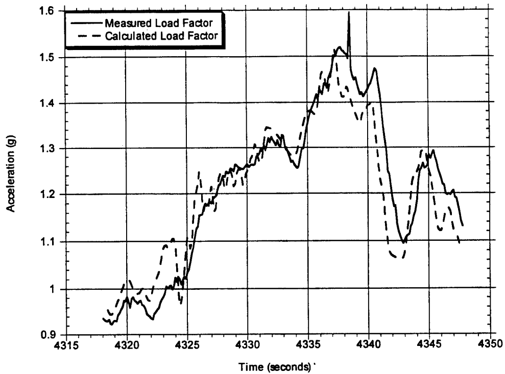
FIGURE 18. COMPARISON OF MEASURED AND CALCULATED LOAD FACTOR
