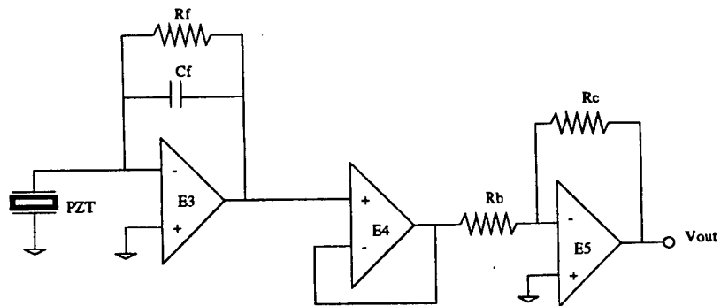
Figure 5: Sensor signal conditioning circuitry
