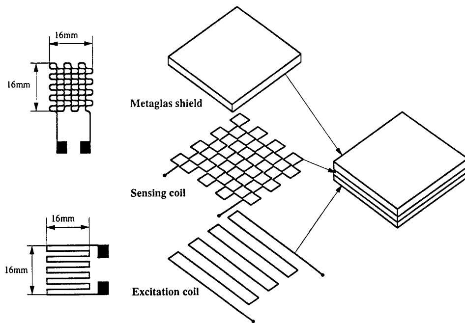
Figure 5. (a) Mesh coil sensor with a 16 mm square planar excitation coil, a planar sensing coil and a Met Glass magnetic shield.
