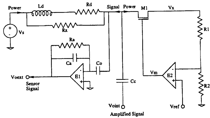
Figure 4: Power regulator and telemetry interface
