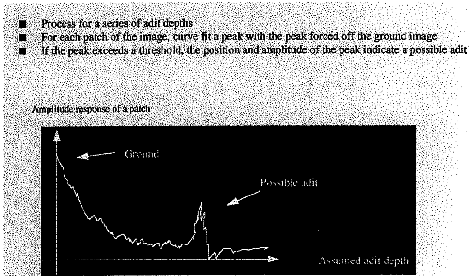
Figure 2-6: Depth algorithm.
