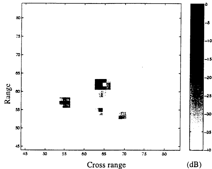
Fig.9. The ISAR image of the blades with the body interference removed.
