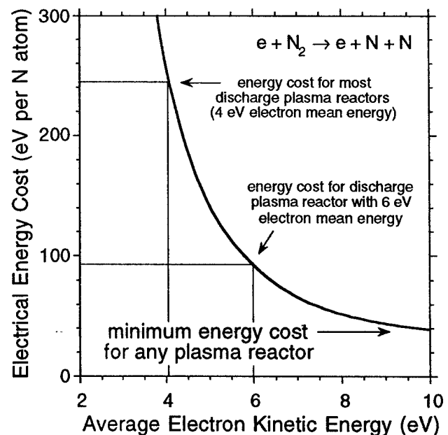
Figure 4. Electrical energy cost for N atom production as a function of the average electron kinetic energy.
