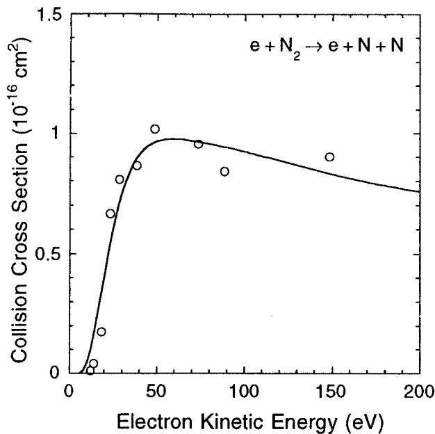
Figure 1. Cross section for electron-impact dissociation of N_2 .
