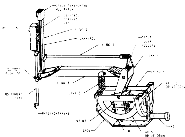
Figure 4: The Black Falcon mechanical overview.
