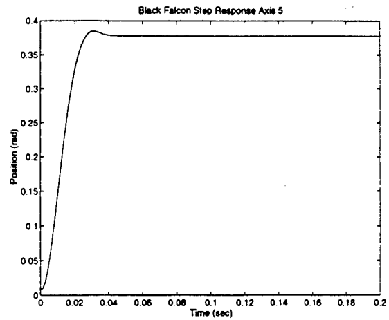
Figure 8-6: Joint 5 response to a 0.4 rad step input.
