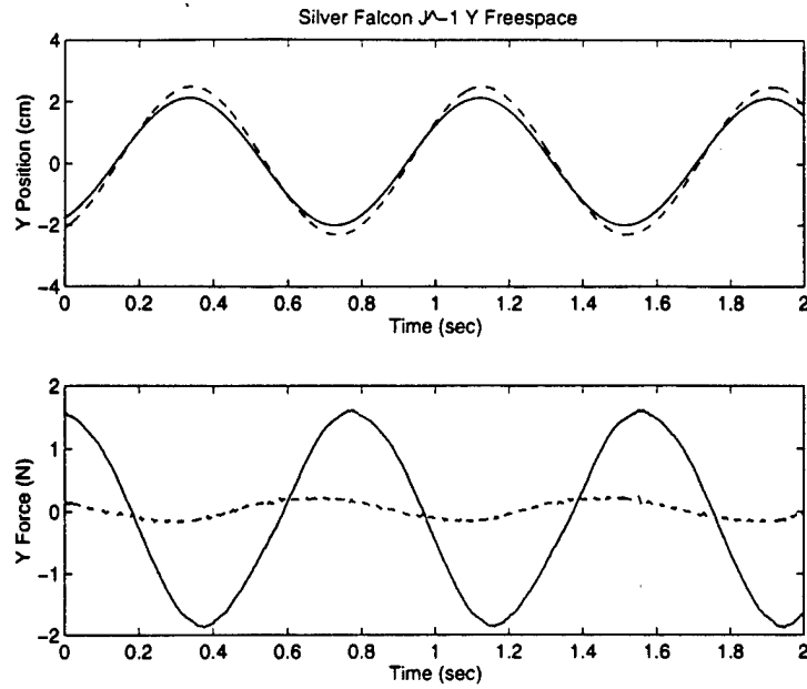
Figure 6-17: Freespace response for the Silver Falcon slave and PHANToM master in the y direction using the Jacobian Inverse controller. The solid line represents the master, and the dashed line represents the slave.
