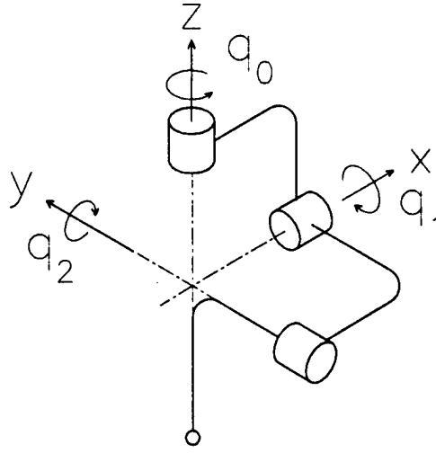
Figure 3-4: Kinematics for a roll-pitch-yaw wrist. The small circle at the lower tip of the structure represents a point where objects might be held by a gripper mounted distally on the wrist.
