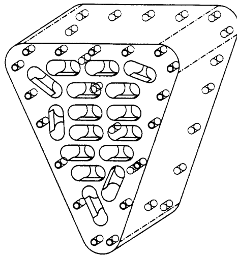
Figure 7-8: The counterweight incorporates radiator like passages for water cooling. It is copper for high thermal conductivity, and use two end plates to form a single continuous water channel.
