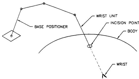
Figure 2: The kinematic constraints on the slave manipulator defines its overall structure. While many other general concepts could be formulated (snake robots, parallel robots which assemble through multiple ports), a slave manipulator which consists of a wrist unit coupled to a base positioner is straightforward and has proven effective.
