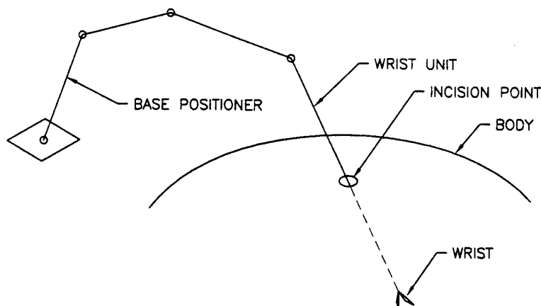
Figure 3-2: The kinematic constraints on the slave manipulator defines its overall structure. While many other general concepts could be formulated (snake robots, parallel robots which assemble through multiple ports), a slave manipulator which consists of a wrist unit coupled to a base positioner is straightforward and will prove effective.
