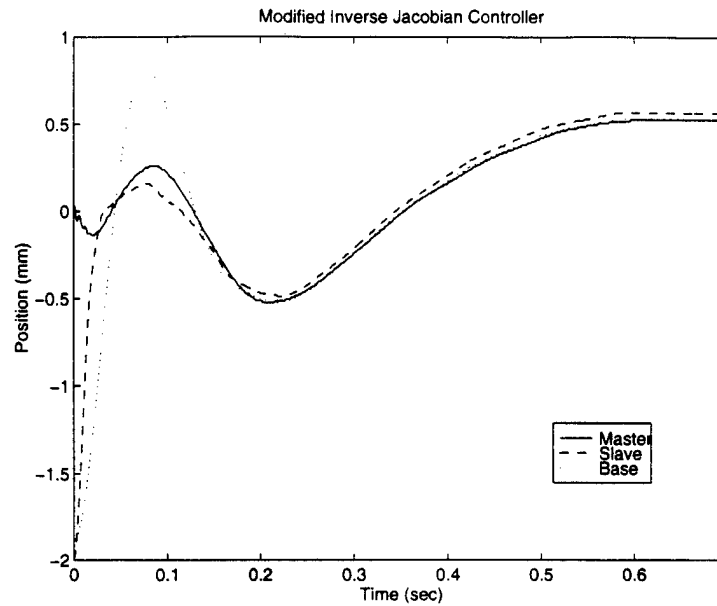
Figure 4-18: Step response for the master and slave using the Modified Jacobian Inverse control.
