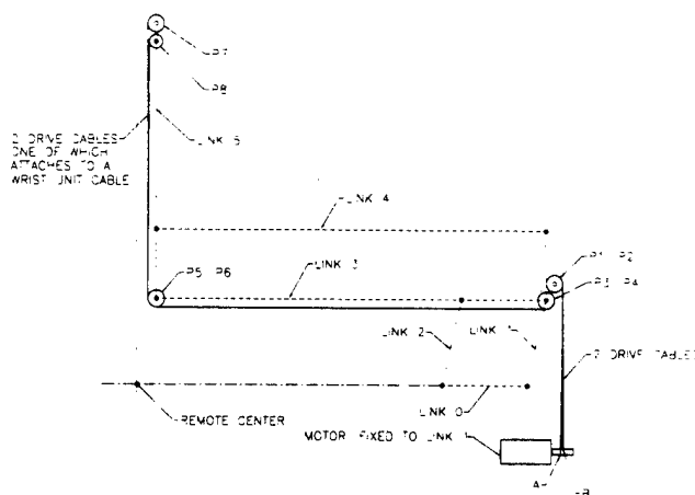
Figure 5: The cabling scheme for the base unit allows it to pitch forward and backward without moving the cables relative to the carriage thereby eliminating coupling. The solid line represent mechanical cables, and the dashed lines represent the structure.
