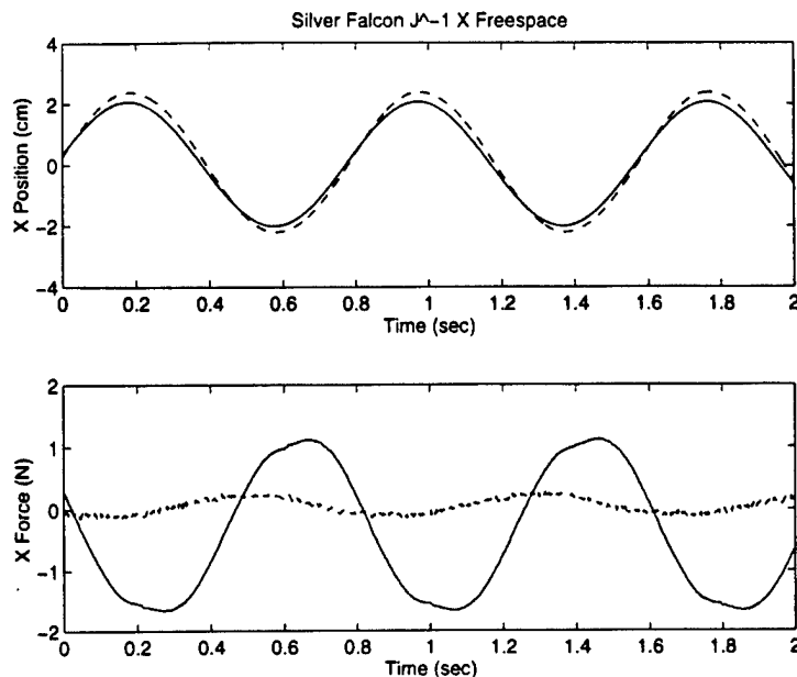
Figure 6-16: Freespace response for the Silver Falcon slave and PHANToM master in the x direction using the Jacobian Inverse controller. The solid line represents the master, and the dashed line represents the slave.
