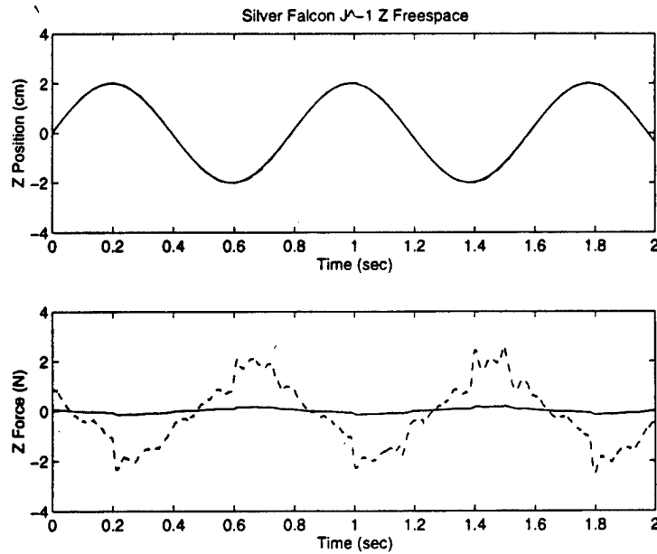
Figure 6-18: Freespace response for the Silver Falcon slave and PHANToM master in the z direction using the Jacobian Inverse controller. The solid line represents the master, and the dashed line represents the slave.
