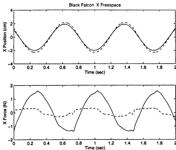
Figure 8-16: Freespace response for the Black Falcon slave and PHANToM master in the x direction using the Inverse Jacobian controller. The solid line represents the master, and the dashed line represents the slave.
