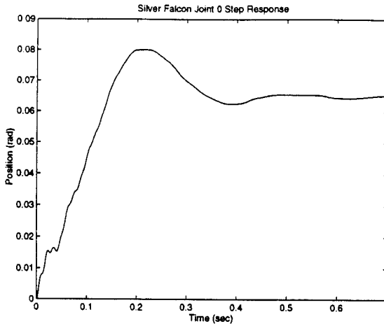
Figure 6-1: Silver Falcon Joint 0 response to a 0.07 rad step input.
