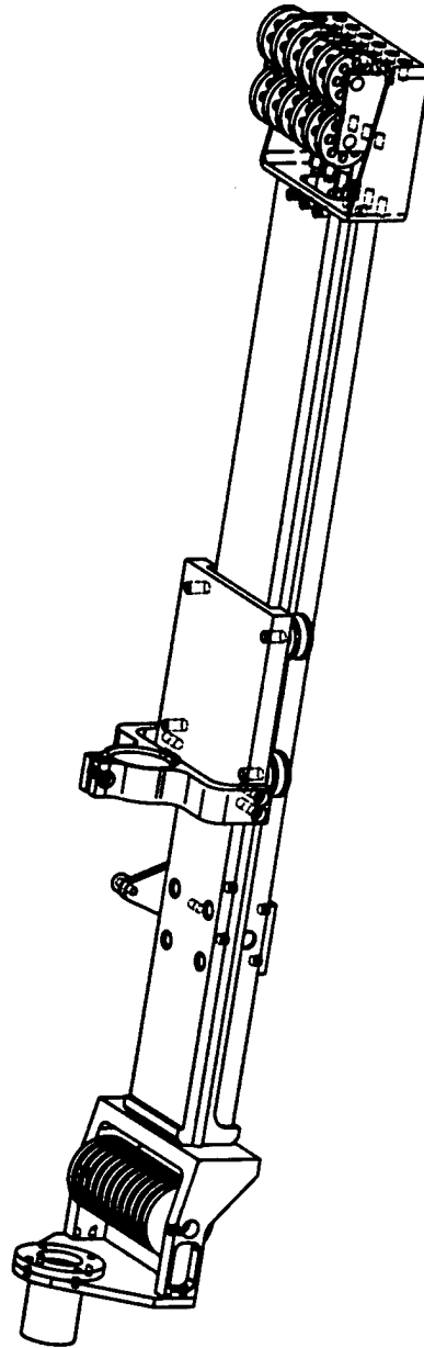
Figure 7-10: The wrist unit is supported on a carriage. This carriage is mounted on INA roller bearings which run on 4 mm steel shafts mounted into grooves machined the carriage beam, which is constructed of machined aluminum box tubing and welded to the lower fork.
