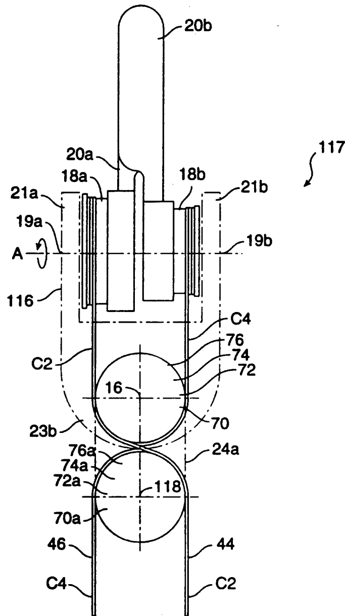
Figure 5-15: N + 1 Cable actuation scheme for the non- \alpha wrist. This wrist reduces friction by avoiding all \alpha -wraps within the wrist. The wrist structure 116 rotates about the axis labeled 16.
