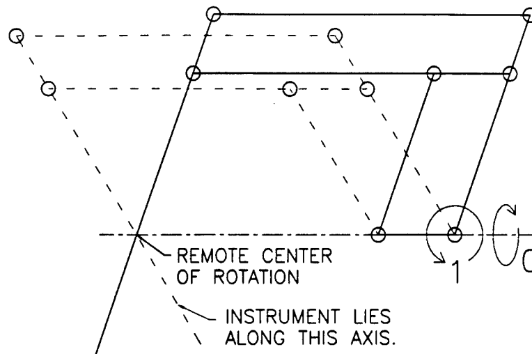
Figure 3-9: The double parallelogram remote center linkage. The circles represent revolute joints whose axes are perpendicular to the page. Axis 0 rotates the linkage out of the plane of the page.
