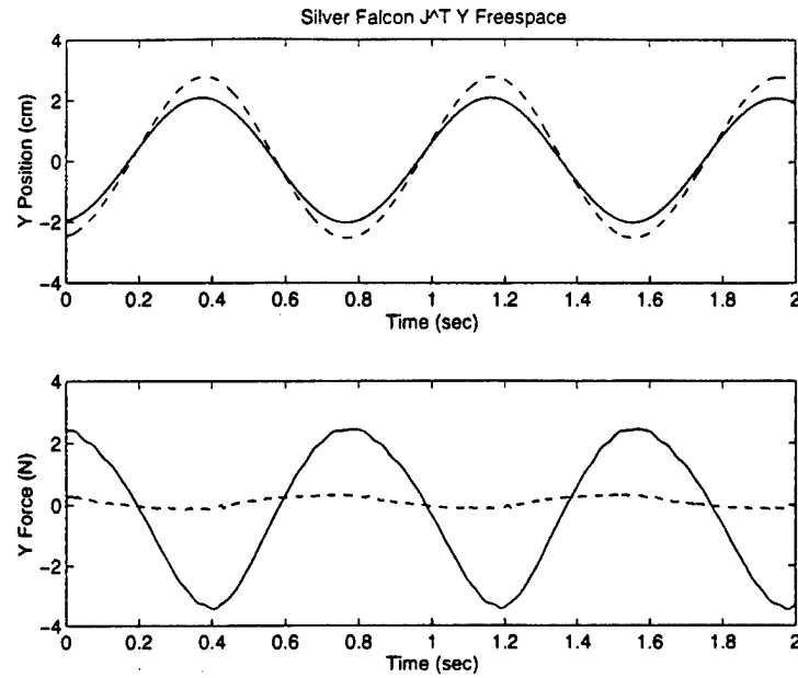
Figure 6-14: Freespace response for the Silver Falcon slave and PHANToM master in the y direction using the Jacobian Transpose controller. The solid line represents the master, and the dashed line represents the slave.
