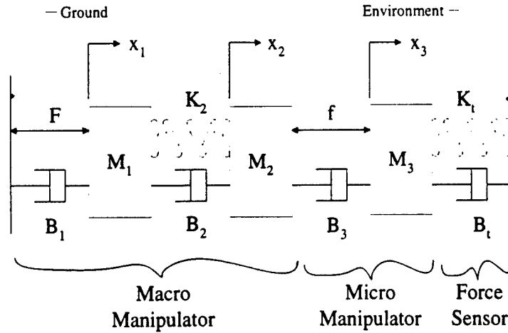
Figure 2-2: Sharon's macro-micro model. The macro manipulator is assumed flexible. K_t and B_t represent stiffness and damping of a force sensor mounted to ground upon which the micro manipulator pressed during force control contact tests.
