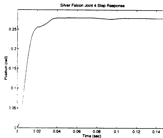
Figure 6-6: Silver Falcon Joint 4 response to a 0.3 rad step input.
