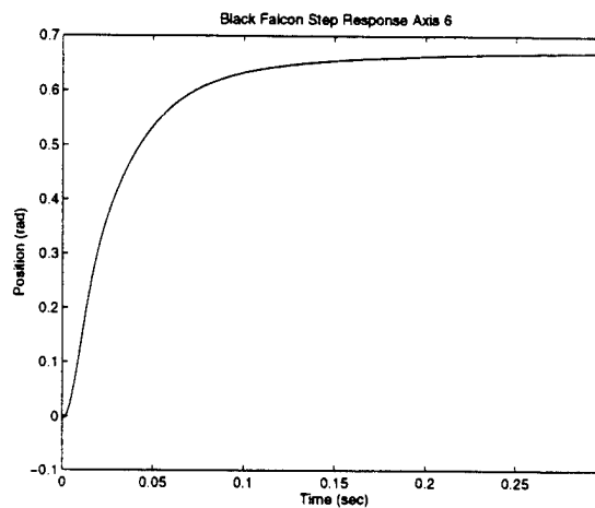
Figure 8-14: Joint 6 response to a 0.8 rad step input. Gains used during force reflection tests.
