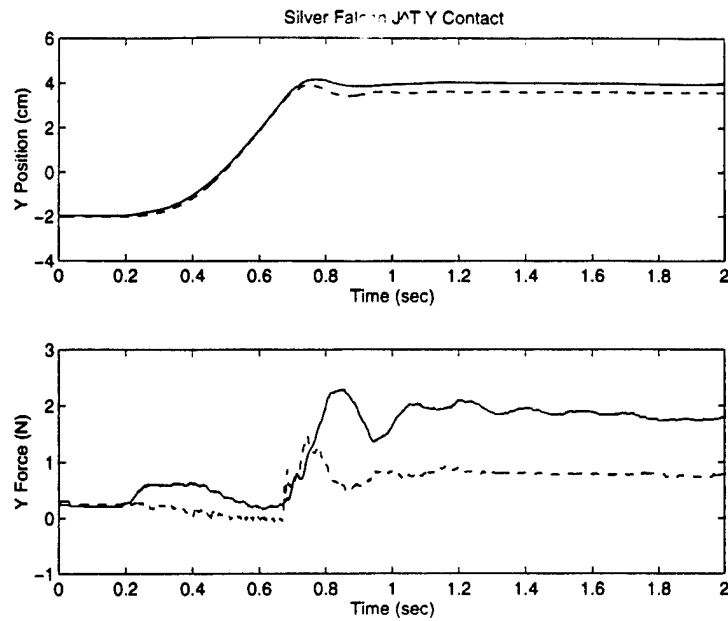
Figure 6-21: Contact response for the Silver Falcon slave and PHANToM master in the y direction using the Jacobian Transpose controller. The solid line represents the master, and the dashed line represents the slave.
