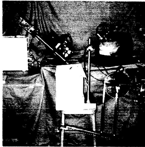
Figure 10: The slave is positioned above chicken tissue which is sitting on several boxes on a stool. The toolhandle master is in the foreground.
