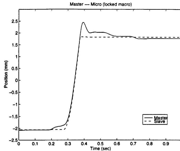
Figure 4-13: Contact response for the master and micro axes slaved together using basic teleoperator control.
