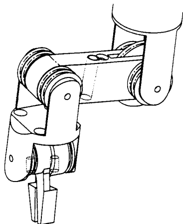
Figure 6: The four-degree-of-freedom wrist.
