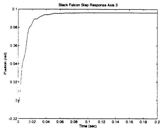
Figure 8-4: Joint 3 response to a 0.1 rad step input.
