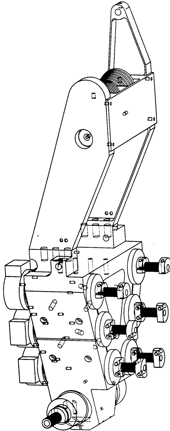
Figure 7-7: Link 1 clamps 7 of the 8 motors in a block machined from a single piece of aluminum. A triangular water-cooled counterweight fits into this piece. Two vertical uprights and a pulley support piece form the remainder of the structure. Each motor is fitted with a threaded cable drive capstan.
