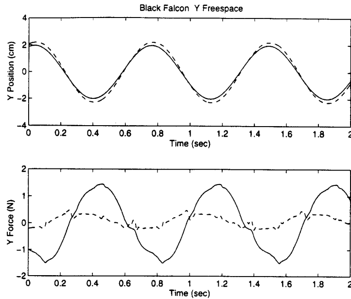
Figure 8-17: Freespace response for the Black Falcon slave and PHANToM master in the y direction using the Inverse Jacobian controller. The solid line represents the master, and the dashed line represents the slave.
