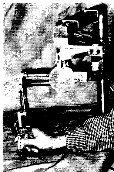
Figure 7: The PHANTOM haptic interface modified for use as master manipulator.
