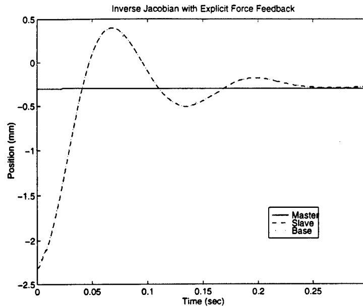
Figure 4-20: Step response for the master and slave using a simulated force sensor controller.
