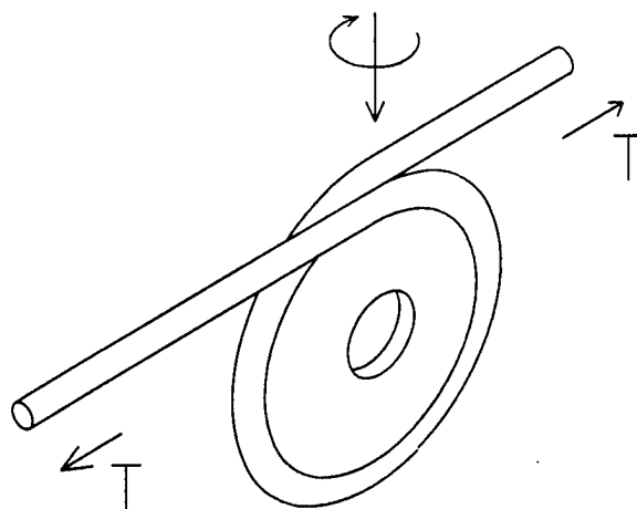
Figure 5-14: The \alpha -wrap causes two problems. (a) the cable rubs on itself, and (b) it causes the pulley to tilt. If T is the tension on the cable, then there is a torque on the pulley equal to T \times d where d is the cable diameter.
