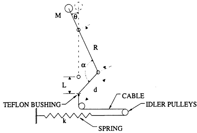
Figure 5-7: The spring counterbalance approximately balances gravity imbalance torques.
