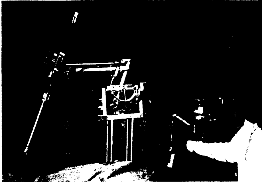
Figure 5-17: The Silver Falcon slave was used in conjunction with the PHANToM haptic interface. An instrumented gimbal and gripper were added to the end of the PHANToM so that it had a total of seven degrees of freedom (3 actuated).
