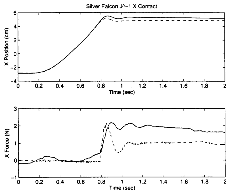
Figure 6-23: Contact response for the Silver Falcon slave and PHANToM master in the x direction using the Jacobian Inverse controller. The solid line represents the master, and the dashed line represents the slave.
