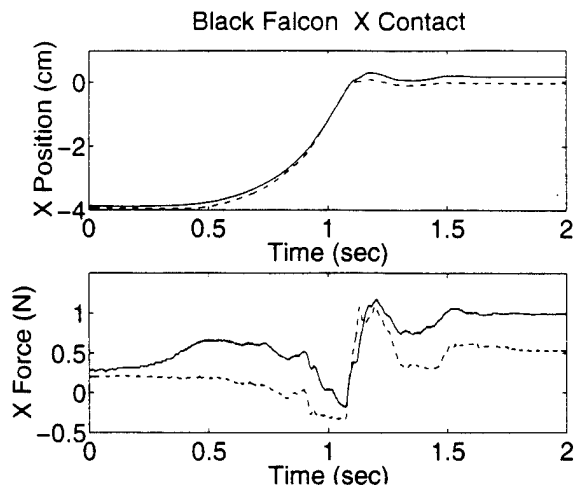
Figure 8: Contact response for the Black Falcon slave and PHANToM master in the x direction. The solid line represents the master, and the dashed line represents the slave. While contact is clear, substantial forces are applied through the master during free space motions. 2:1 force scaling is implemented.
