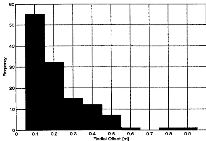
Figure II-54. Common Detection Radial Location Offset
