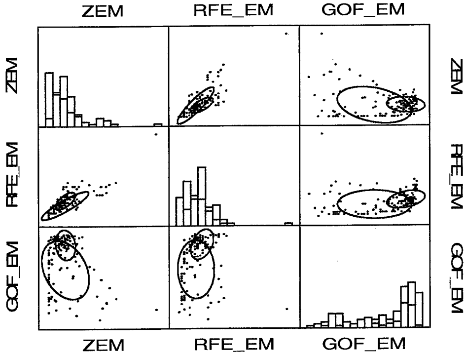
Figure II-22. Scenario 2 Correlation of EMI Variables. Blue = False Alarms. Red = Detections. 50-percent ellipses are shown.
