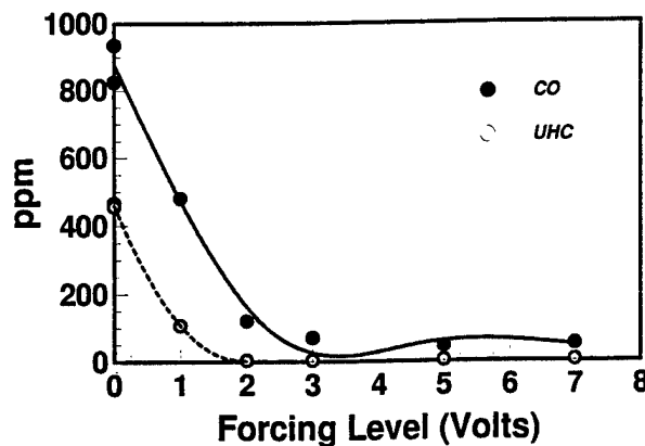
Fig. 15 Effect of forcing level on CO and UHC emissions (uncorrected for O 2 %).
