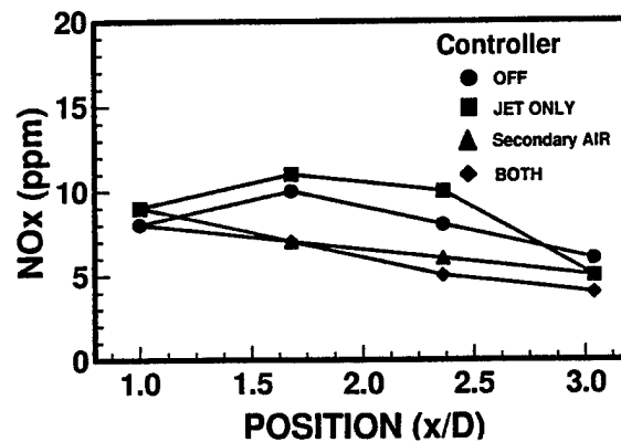
Fig. 6 NO x vs. downstream distance.
