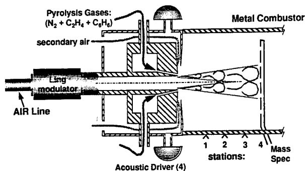
Fig. 3 Version 5 of the 50 kW afterburner. The waste surrogate flow is not directly forced but is sandwiched between the main air shear layer and the acoustically forced secondary entrainment air flow.
