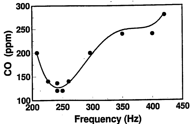
Fig. 14 Effect of forcing frequency on CO emissions from 380 kW enclosed afterburner. The minimum emissions occur at the preferred mode of the air jet.
