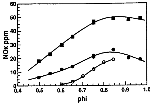
Fig. 9 NOx vs. fuel to air stoichiometry for the controller off (■), on at 11 volts (●), and on at 22 volts (○).
