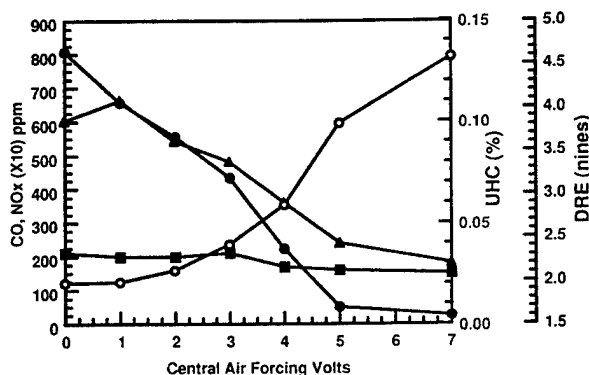
Fig. 7 Benzene DRE (in nines, right axis, ○), unburned hydrocarbons (UHC axis on right, ▲), CO ppm (●), and NO_x ppm times 10 (■) for the afterburner configuration shown as a function of forcing level on the controller. As control authority is exercised the benzene DRE goes up and the CO, UHC, and, to some extent, the NO_x go down.
