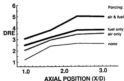
Fig. 4 Benzene DRE (in nines) as a function of axial position x/D (where x is the axial distance downstream from the dump and D is the dump diameter) for various conditions of the GB controller. The top curve is the entire controller optimized; the next down is for forcing of the fuel jets only; the next for air forcing only; and the bottom for no forcing at all.
