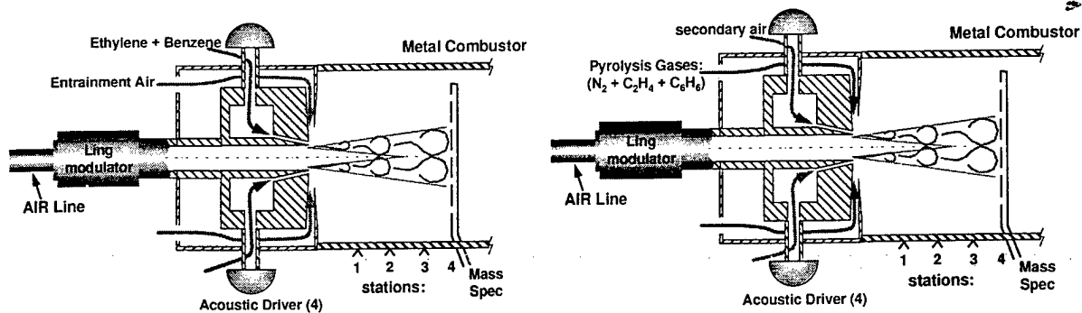
Fig. 1 Schematic diagram of the 50 kW actively controlled dump combustor incinerator afterburner concept: (a, left) Gas Burner (GB) configuration, (b, right) After Burner (AB) configuration.
