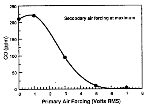
Fig. 6 CO (in ppm) versus central air forcing level (Vling in volts RMS) in the original AB configuration.
