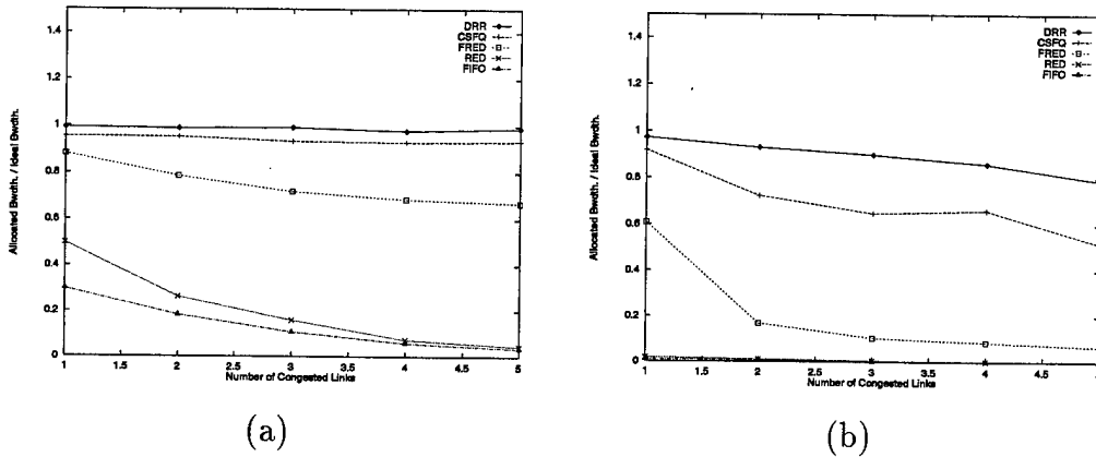
Figure 7: (a) The normalized throughput of UDP-0 as a function of the number of congested links. (b) The same plot when UDP-0 is replaced by a TCP flow.
