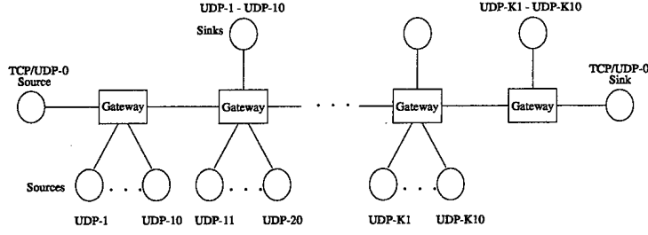
Figure 6: Topology for analyzing the effects of multiple congested links on the throughput of a flow. Each link has ten cross flows (all UDPs). All links have 10 Mbps capacities. The sending rates of all UDPs, excepting UDP-0, are 2 Mbps, which leads to all links between routers being congested.
