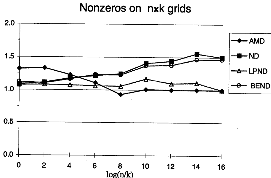
Figure 1.1: Number of nonzeros introduced by different elimination orders for n \times k rectangular grids relative to a special-purpose order.
