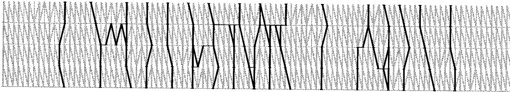
Figure 5.1: Partial elimination of a graph, according to a BEND order.
