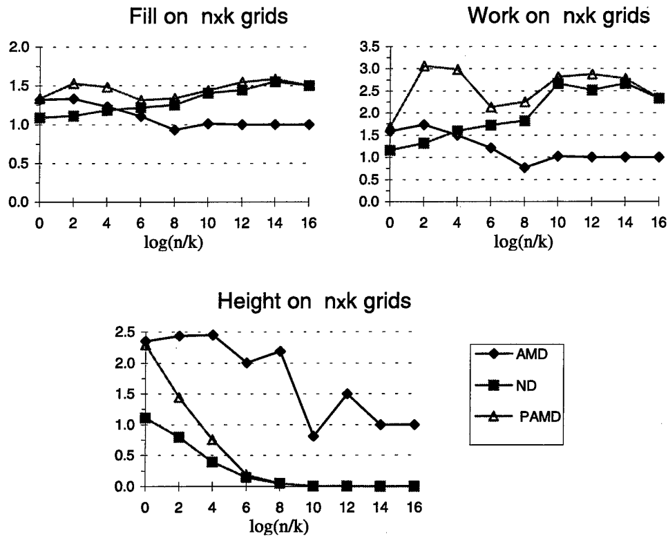
Figure 5.2: Comparison between orders produced by nested dissection (ND), minimum-degree (AMD), and the order obtained by applying the parallelizing algorithm of the previous chapter as a post processing step to the AMD order (PAMD).
