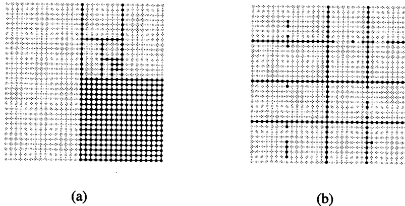
Figure 3.3: Partial elimination according to a nested dissection order.
