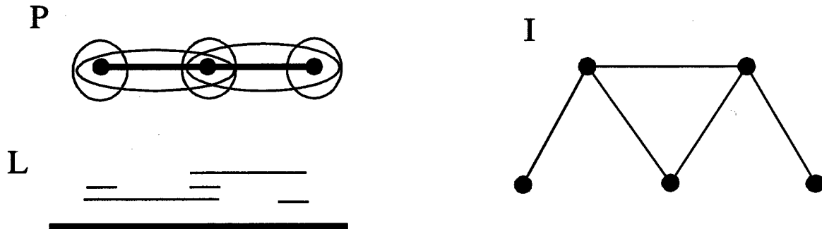
Figure 2.4: Representations of an interval graph I as an intersection graph.
