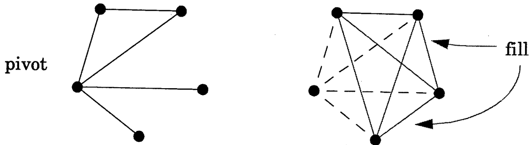
Figure 2.1: The elimination of the vertex corresponding to the pivot in a given step introduces fill edges between its neighbors.
