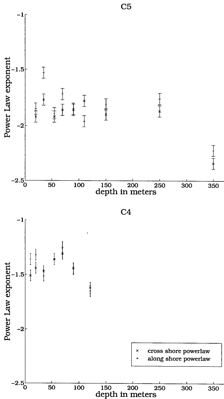
Figure 5.8: Slope of the power spectrum of each current meter in log/log space. The top plot is from C5 and the bottom from C4.
