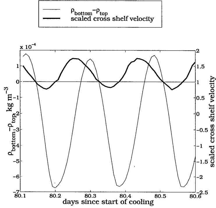
Figure 2.9: \rho_{bottom} - \rho_{top} and scaled near bottom cross-shelf velocity 17 km offshore of the coast. The model is run with a 0.1 \text{ N m}^{-2} alongshore upwelling favorable wind.
