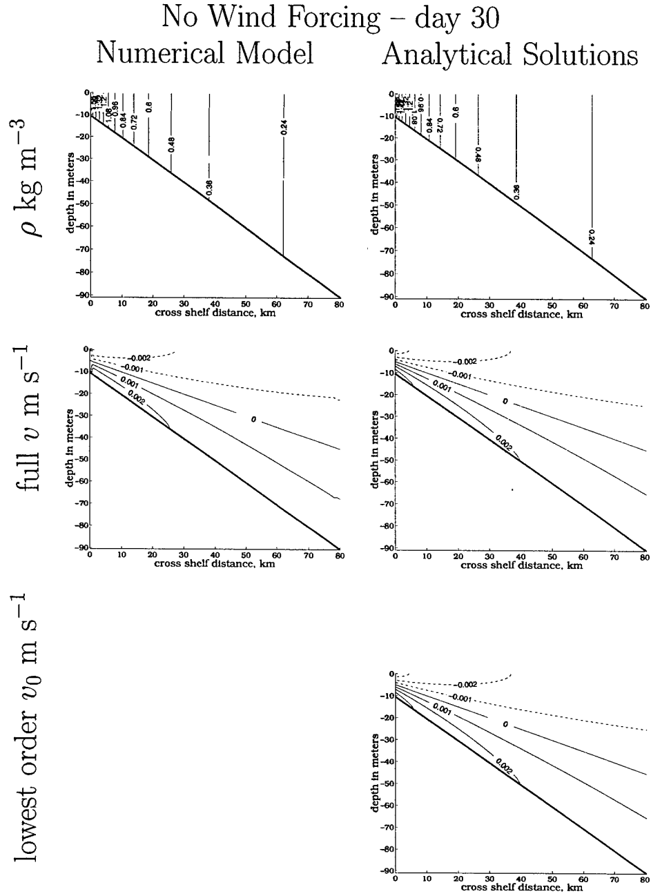
Figure 2.3: The solutions for the cross-shelf velocity and the density from (2.14), (2.5) and the numerical model. The bottom panel is the lowest order analytic solution for the cross-shelf flow. Dashed contours are negative.
