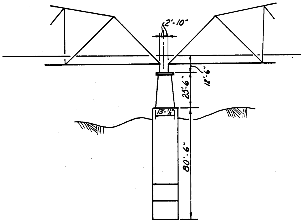
ELEVATION VIEW
