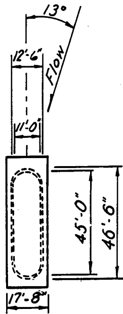
PLAN VIEW
