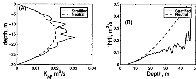
Figure 5.14: A comparison of the neutral (unstratified) downwelling case and the downwelling base case, at 9 days. (A) Profiles of eddy viscosity 25 km offshore; (B) the maximum streamfunction as a function of local water depth.
