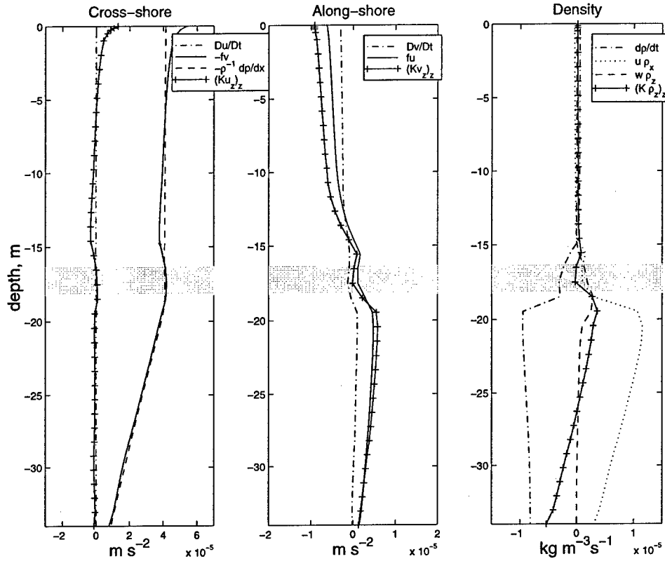
Figure 5.16: Terms of the cross-shelf momentum balance, alongshelf balance, and density balance in the frontal region, at 30 km offshore at 4.5 days. The shaded region represents the vertical range of strong vertical stratification ( \frac{d\rho}{dz} > 0.05 \text{ kg m}^{-3} ).
