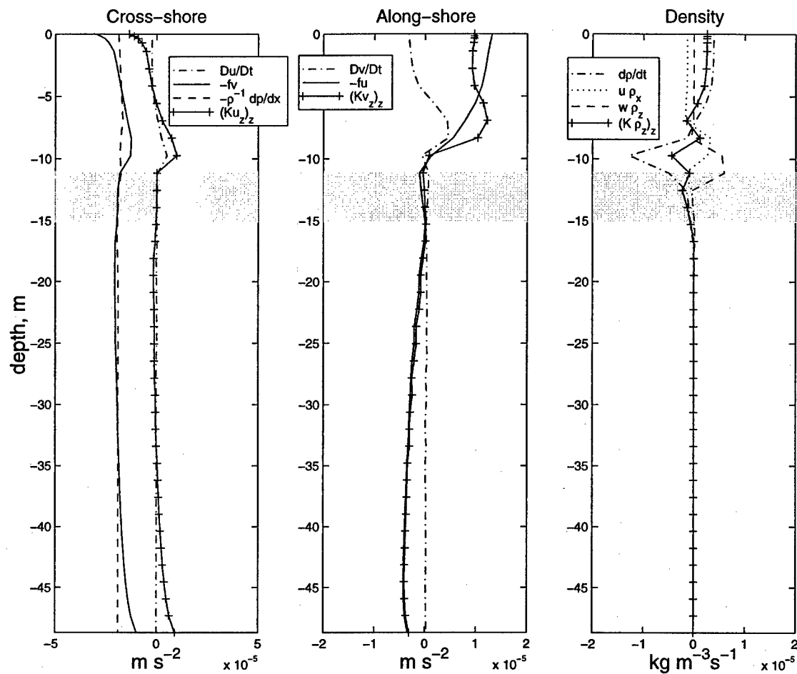
Figure 4.17: Cross-shelf, alongshelf, and density balances from the mid-shelf (45 km offshore, 2.5 days) in the base case. The shading represents the depth range of strong vertical stratification ( \frac{d\rho}{dz} > 0.05 \text{ kg m}^{-3} ).
