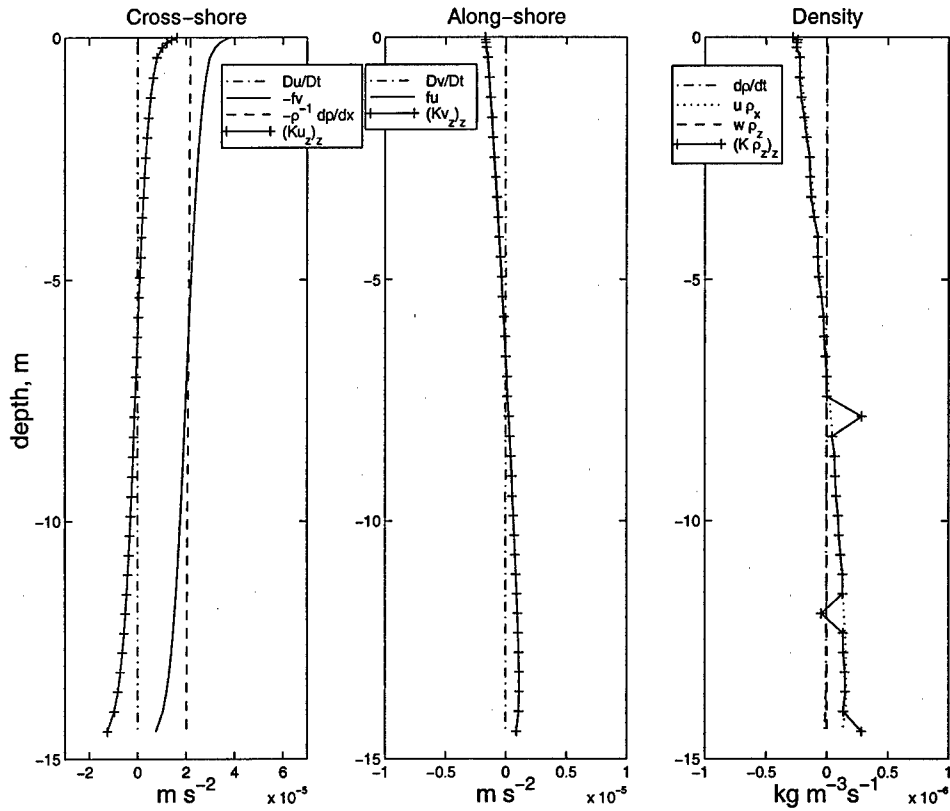
Figure 5.10: Terms of the cross-shelf momentum balance, alongshelf momentum balance, and density balance on the inner shelf, at 10 km offshore at 4.5 days. The “spikes” in the density mixing profile at 8 m and 12 m are balanced by the horizontal diffusivity (not shown).
