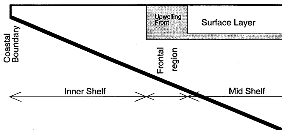
Figure 4.6: A schematic of the shelf during an upwelling event, defining some of the basic terms used. The shaded region represents the pycnocline and the upwelling front.
