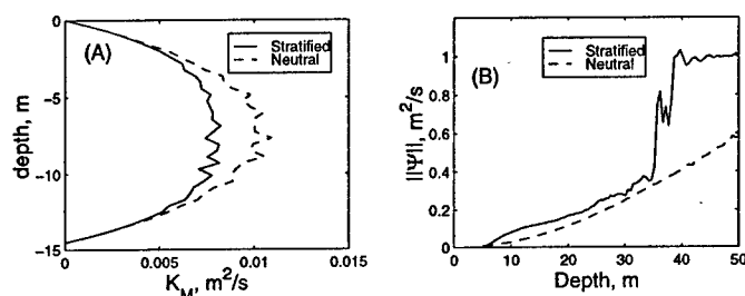
Figure 4.10: A comparison of the neutral (unstratified) upwelling case and the upwelling base case (strong pycnocline). (A) Profiles of eddy viscosity 10 km offshore; (B) the maximum streamfunction as a function of local water depth.
