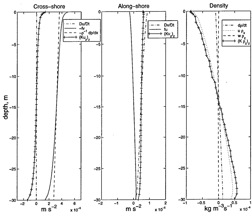
Figure 5.15: Terms of the cross-shelf balance, alongshelf balance, and density balance on the adjusting inner shelf, at 24 km offshore at 4.5 days.
