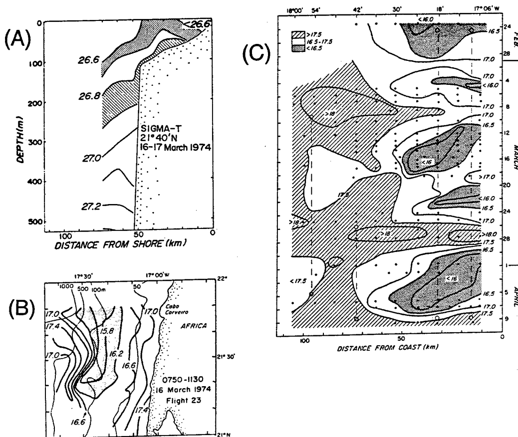
Figure 4.29: Taken from Barton et al. [1977]. Data from the JOINT-1 experiment. A. Density section from 16 March. B. Surface temperature from 16 March. C. Surface temperature as a function of time at 21°40'N.
