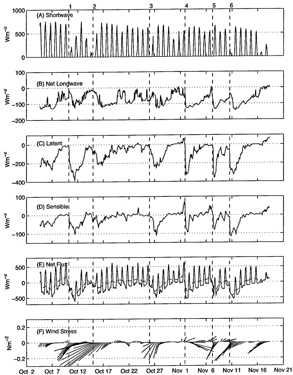
Figure 2.5: Terms of the heat flux and wind stress for the October time period, as in Figure 2.4.
