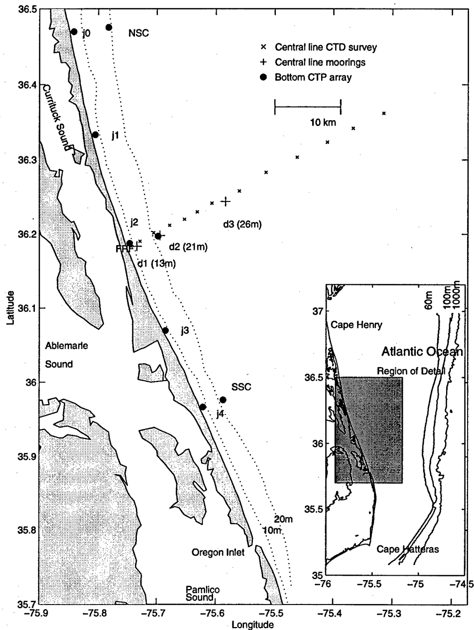
Figure 3.1: The CoOP Inner Shelf Study experimental region, with mooring locations and central line CTD stations specified. Inset is a regional view, showing Cape Henry, at the mouth of the Chesapeake Bay, and Cape Hatteras.
