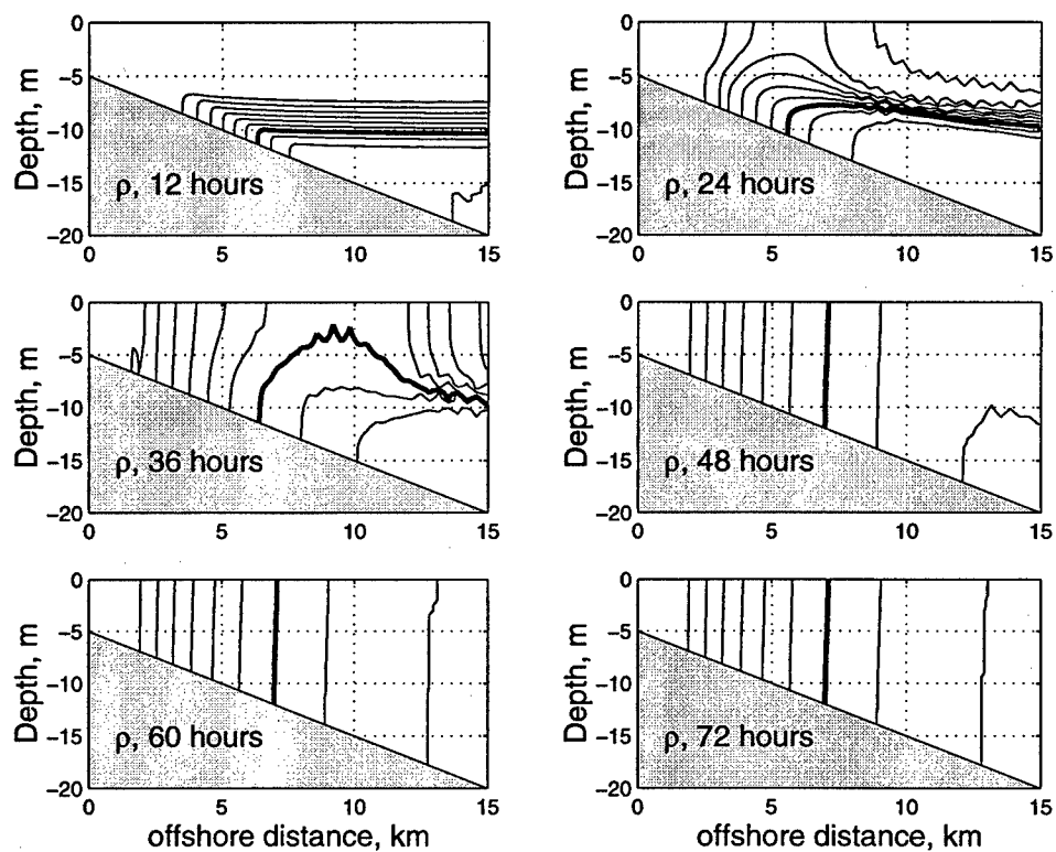
Figure 4.7: The density field at 12 hour intervals, showing the development of the inner shelf region. The heavy line is a fixed \sigma_\theta contour, made distinct so that it can be followed.
