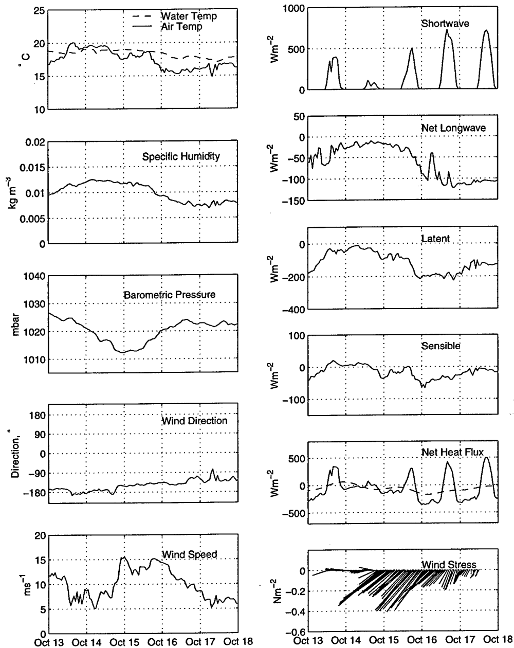
Figure 2.12: Time series of meteorology and surface heat flux terms for the October 15 event.
