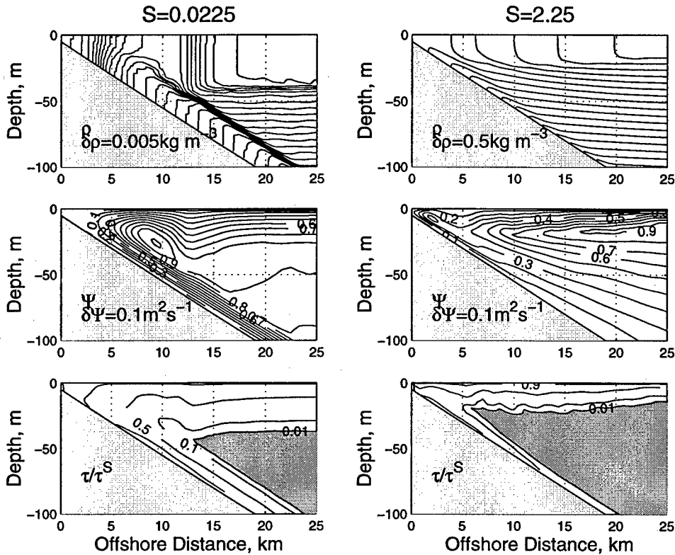
Figure 4.25: Density and cross-shelf streamfunction, at 4.5 days for two continuously stratified runs with different N . The bottom slope is \alpha = 0.005 . Column 1: N = 0.003\text{ s}^{-1} , S = 0.0225 . Column 2: N = 0.03\text{ s}^{-1} , S = 2.25 .
