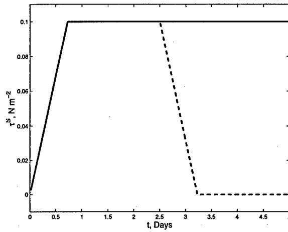
Figure 4.2: The time series of \tau^{SFC} in the constant-stress case (solid line) and the episodic wind case (dashed line).
