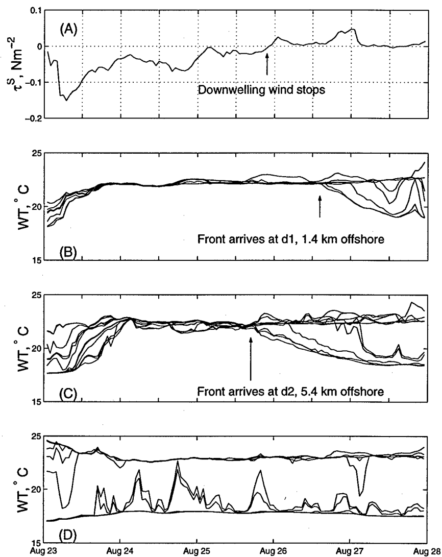
Figure 5.22: Detail of Figure 3.3, during the downwelling event of August 23-27, 1994. A. Alongshelf component of wind stress. B. 6 Temperature records from d1. C. 12 temperature records from d2. D. 10 Temperature records from d3.
