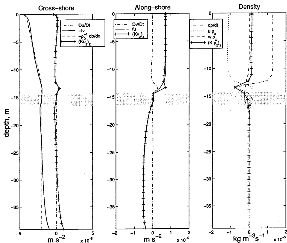
Figure 4.13: Cross-shelf, alongshelf, and density balances from the frontal region (38 km offshore, 4.5 days). The shaded region represents the depth range with strong vertical stratification ( \frac{d\rho}{dz} > 0.05 \text{ kg m}^{-3} \text{ m}^{-1} ).
