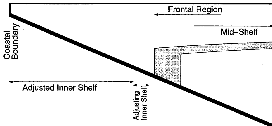
Figure 5.2: Definition of terms referred to in the regional analysis.
