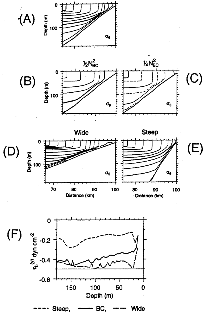
Figure 4.27: Model fields from Allen et al. [1996], all taken after 16 days of \tau^S = 0.05 \text{ N m}^{-2} . \|S\| refers to the maximum Burger number throughout the water column. A. The density field in the base case, \|S\| = 1.8 . B. Density in a weakly stratified case, \|S\| = 0.9 . C. Density in an even more weakly stratified case, \|S\| = 0.45 . D. Density at in a wide-shelf case, \|S\| = 0.45 . E. Density in a steep-shelf case, \|S\| = 7 . F. Bottom stress in the Steep, Base-case, and wide shelf cases.
