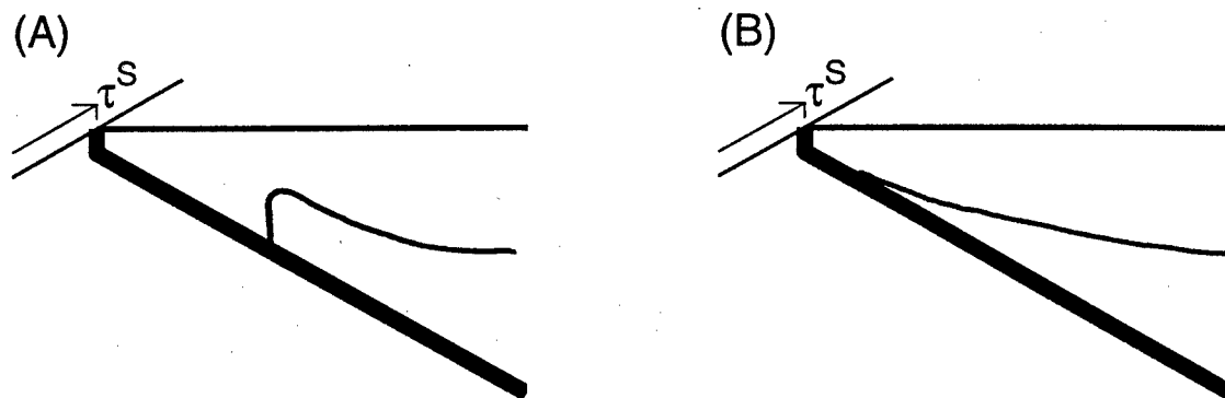
Figure 4.24: Schematic of isopycnal displacement in two different cases: (A) onshore flow due to bottom Ekman layer; (B) onshore flow due to interior flow.
