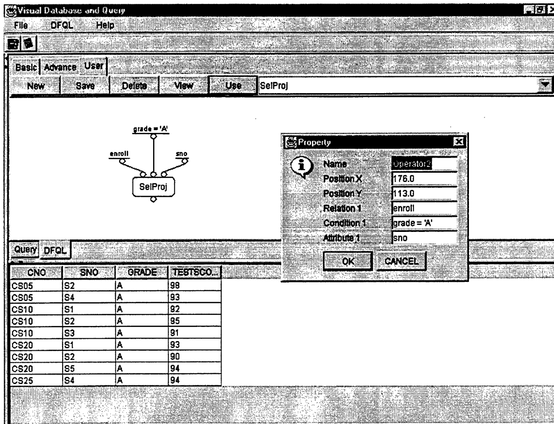
Figure 40. Use and Run the User Defined Operator
