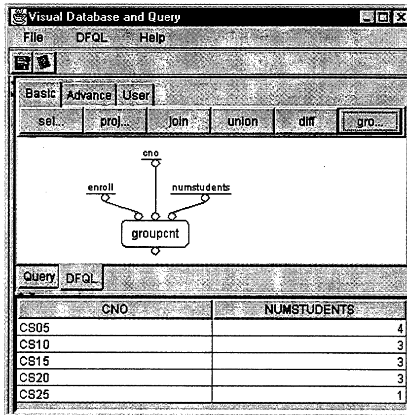
Figure 28. Execution of DFQL operator – Groupcnt
