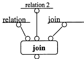
Figure 3: Join operator
