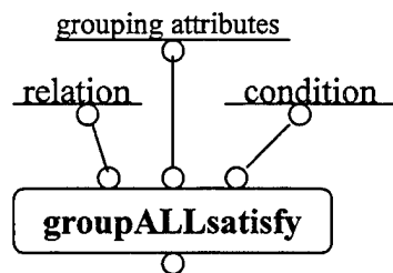
Figure 7: GroupALLsatisfy operator
