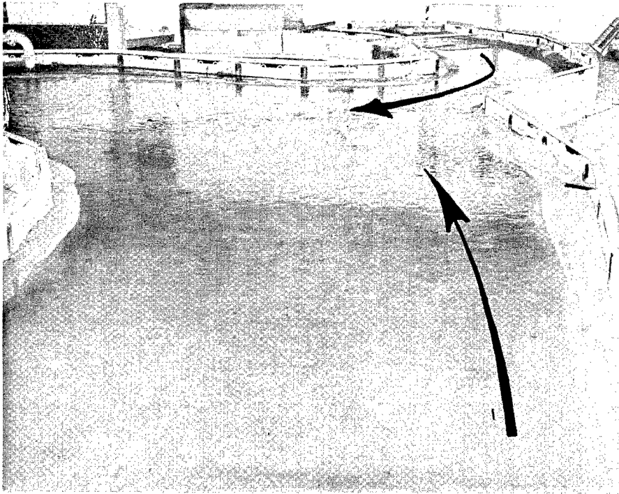
Figure 4. View of model in operation, looking downstream on Missouri River toward confluence.
