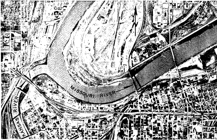
Figure 1. Photograph of the Kansas-Missouri River confluence. Photo indicates the approximate limits of the region used in the model investigation.
