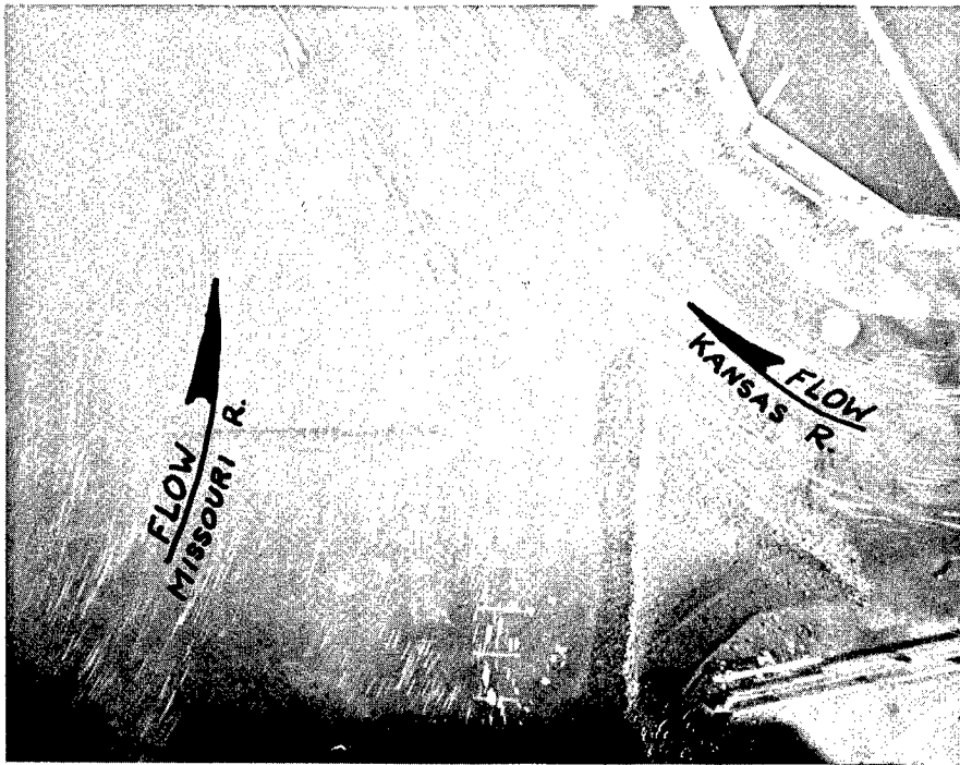
Figure 13. Photograph of structure tested at the confluence and resulting surface currents. Test 300D(L 2 ).
