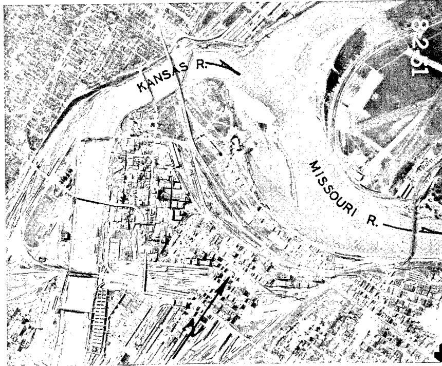
Figure 5. Photograph of the Kansas-Missouri confluence after the 1951 flood. Note large amount of deposition immediately downstream of junction in Missouri River channel.
