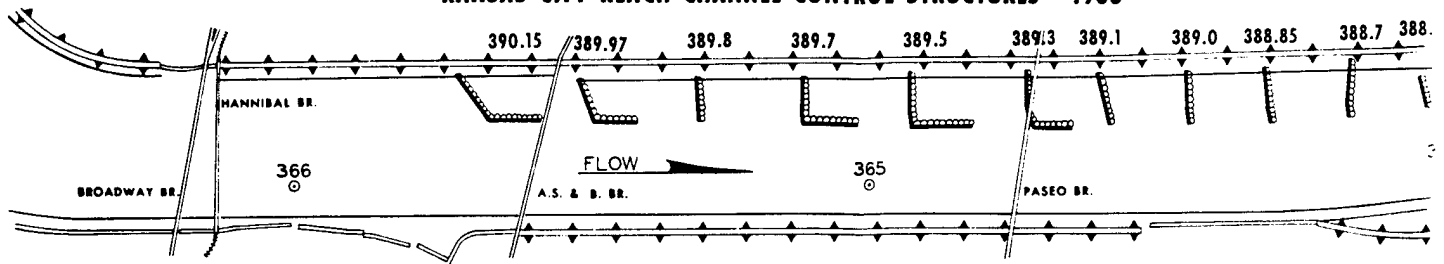
MODEL TEST 26A REPRESENTS 650FT. CONFINEMENT
