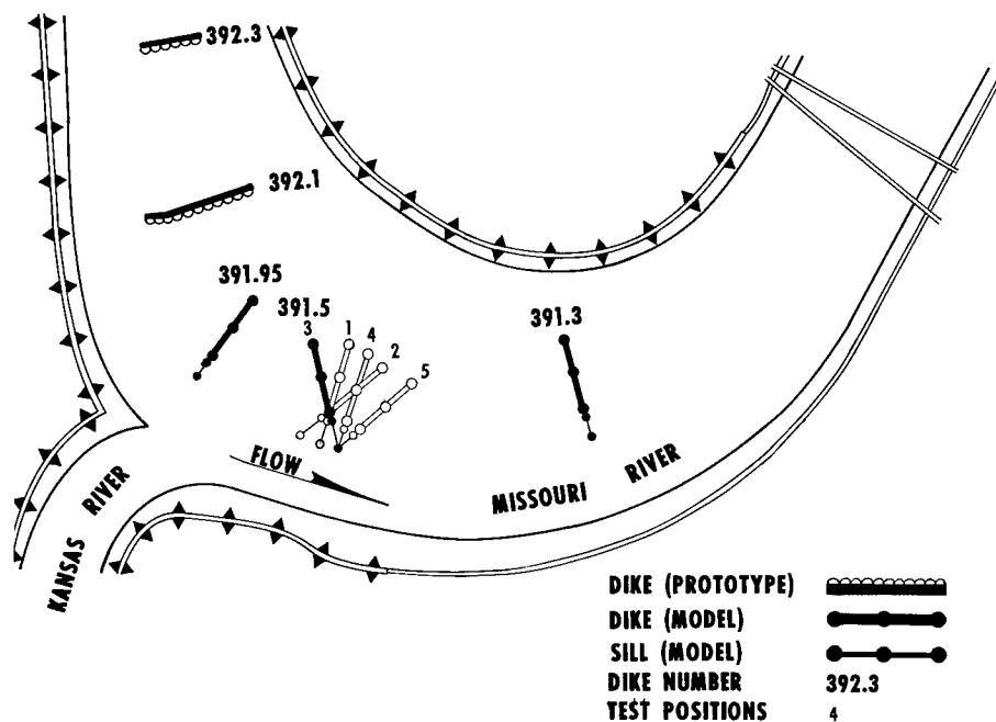
Figure 6. Test Locations for Dike and Sill 391.5.
