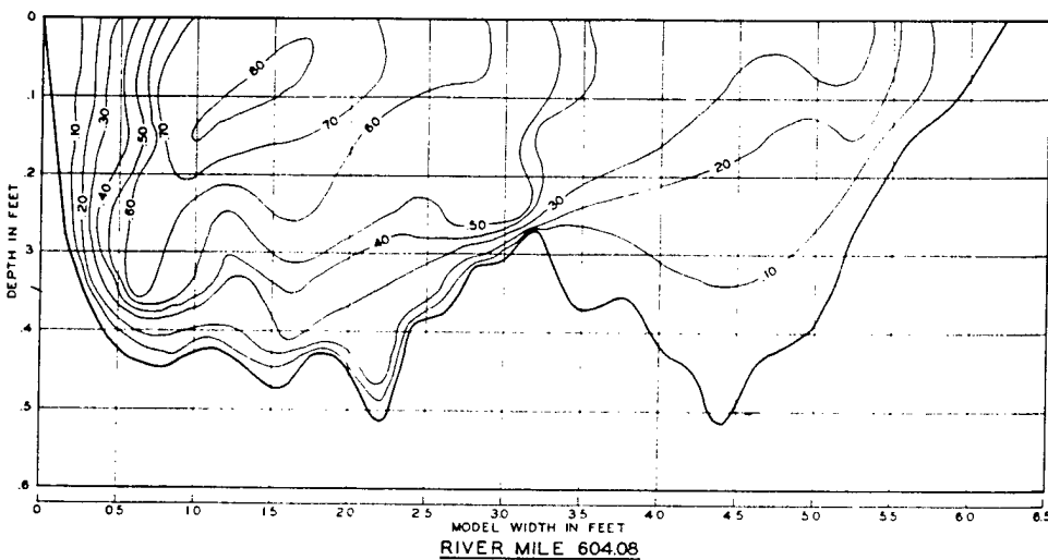
VELOCITY DISTRIBUTION
