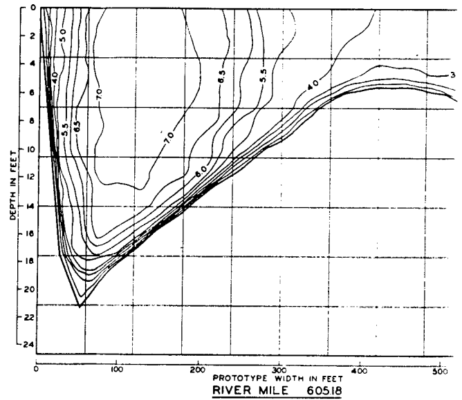
DISCHARGE DISTRIBUTION
