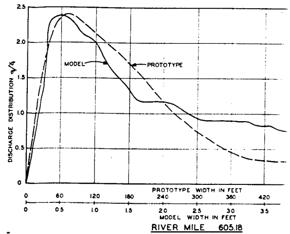
DISCHARGE DISTRIBUTION
