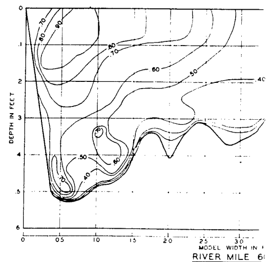
VELOCITY DISTRIBUTION
