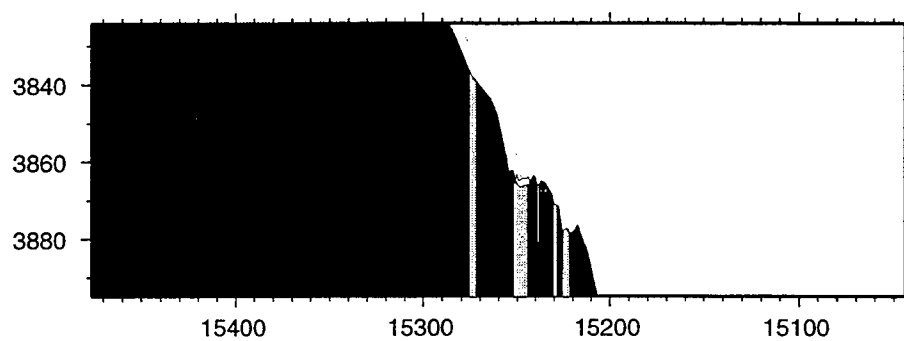
Model 3 with Fracture Heterogeneity
