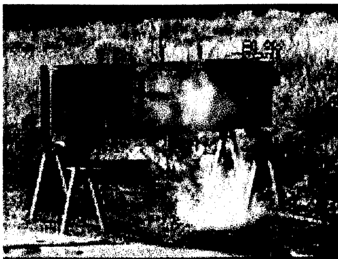
Figure 11. One thirtieth of a second (one frame) following injection of PBr_3 we see evidence of suppression in white smoke on the right half of the bay.
