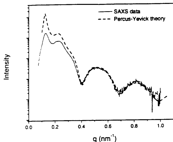
Figure 7. SAXS pattern from an epoxy nanocomposite containing 6 wt % symmetric PEP-PEO diblock copolymer. Close agreement between the experimental and calculated curves confirms a random distribution of nearly monodisperse domains.
