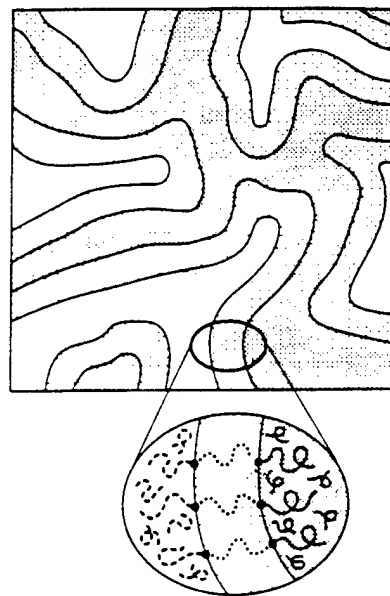
Figure 3. Tricontinuous microemulsion predicted for ternary mixture of ABC triblock copolymer and A' and C' homopolymer (from ref. 19).
