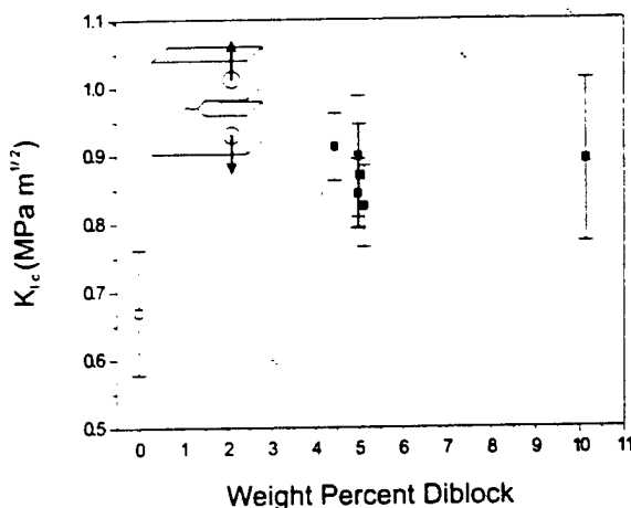
Figure 8. Compact tensile fracture test results for pure epoxy ( \square ) and nanocomposites ( \square ) containing spherical PEP-PEO micelles. Each data point was determined from six fracture tests, except the 10% point which contains three experiments. Five molecular weights, from 2 \times 10^3 to 8.7 \times 10^4 g/mol are represented.
