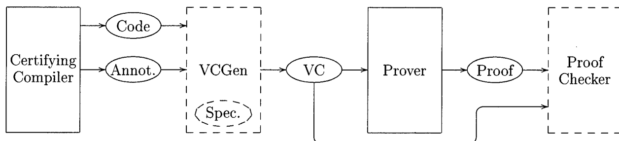
Figure 6.1: The interaction between the PCC tools (shown with continuous lines) and the PCC infrastructure (shown with interrupted lines).
