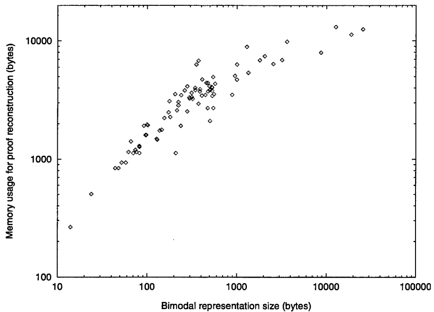
Figure 8.10: The correlation of the memory usage during reconstruction with the size of the bimodal representation, on a logarithmic scale.
