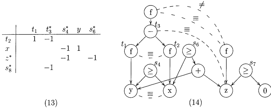
Figure 7.17: State history of the congruence closure and Simplex decision procedures (III).
