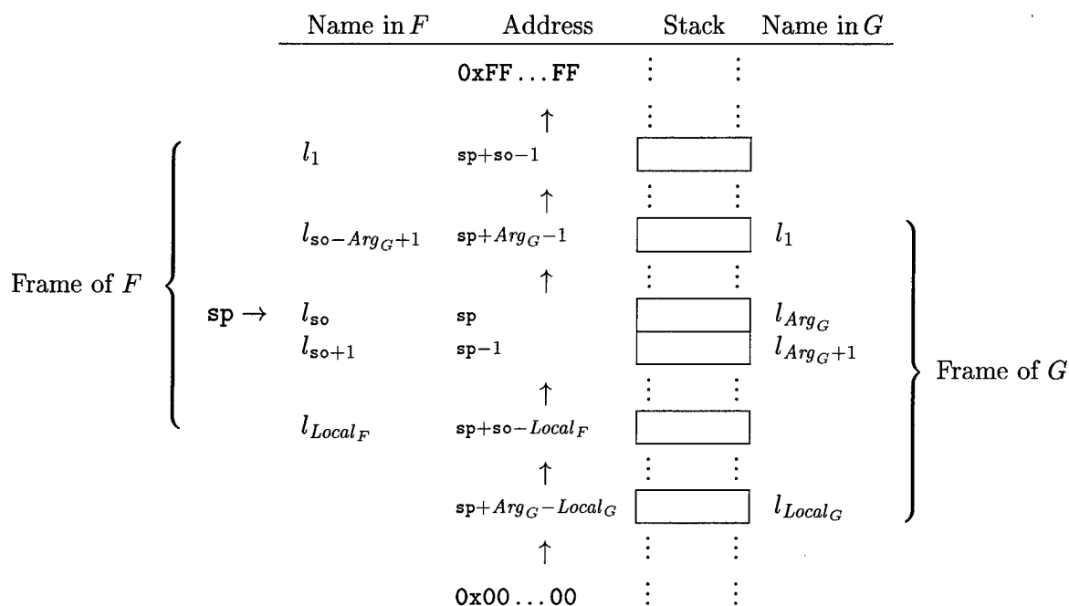
Figure 4.5: Stack management in SAL. The situation depicted occurs at the time when function F calls function G . The value of sp at the time of the call (somewhere in the stack frame of F ) marks the position of the last argument of G , and implicitly defines the alignment of G 's stack frame relative to F 's stack frame. Note the implicit renaming of local pseudo-registers during the call.
