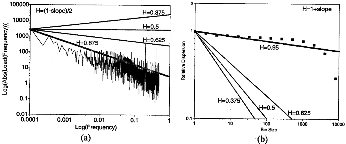
Figure 12: Meaning of the Hurst parameter: (a) Frequency domain interpretation using power spectral analysis, (b) Effect of increased smoothing using dispersal analysis.
