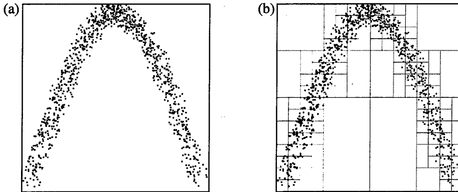
Figure 1: (a) Data set (b) partitioned by a density tree.
