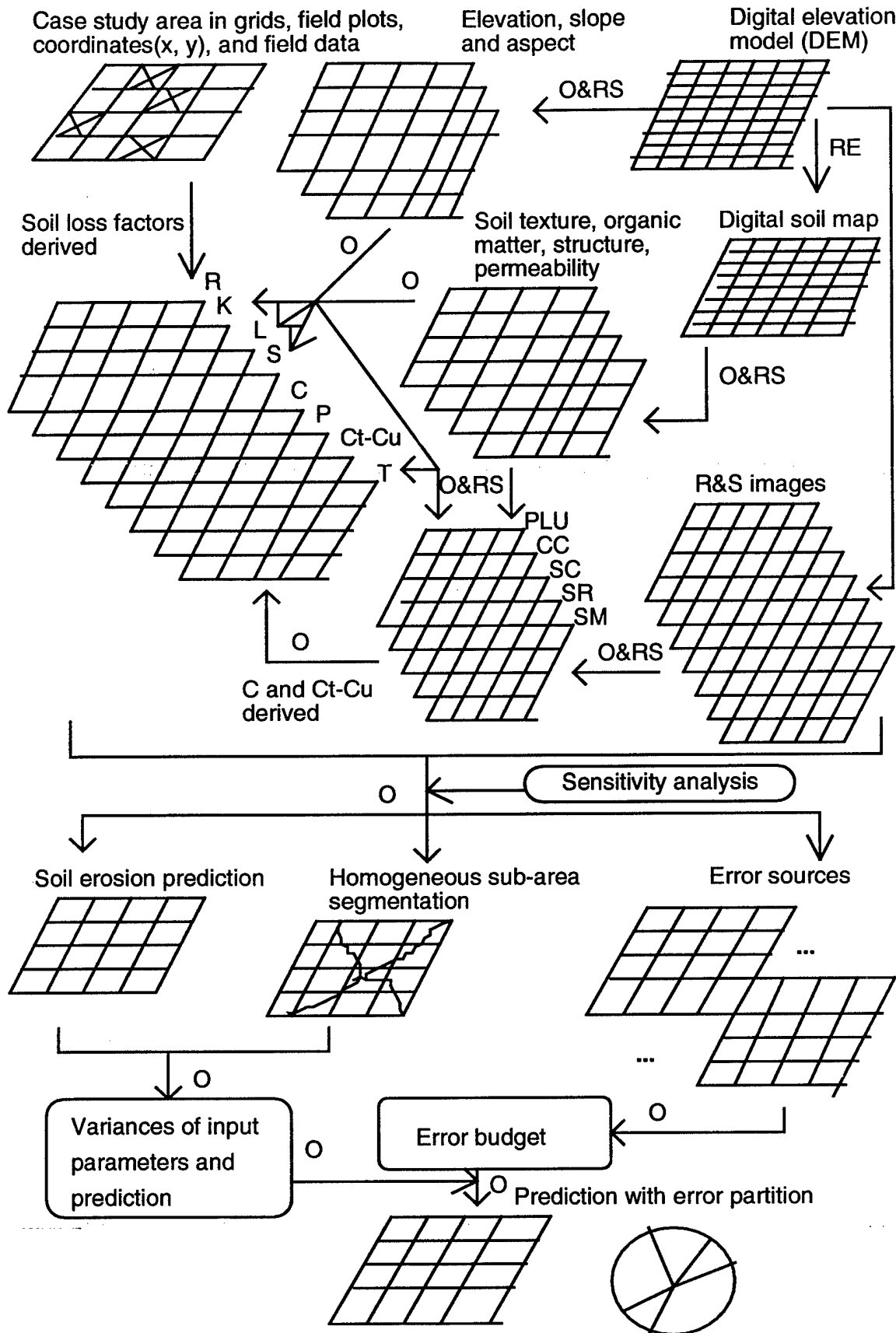
Figure 2. Flow of GIS-based prediction, uncertainty analysis and error budget of soil erosion status (O = operations of image process and statistic, RS = re-sampling, RE = rectification, R&S = remote sensing).
