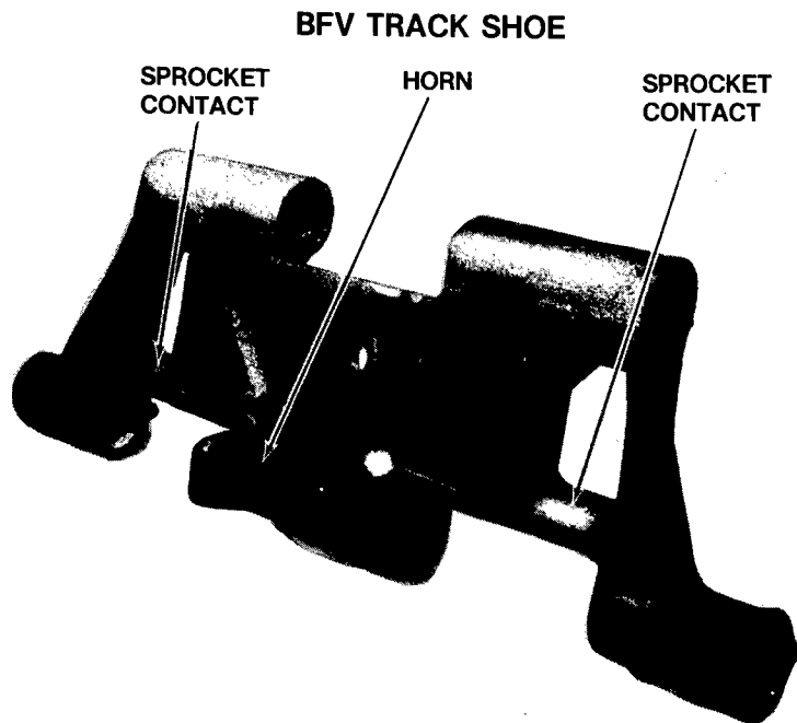
Figure 1 - Sprocket contact and horn regions of track shoe that are surface hardened
