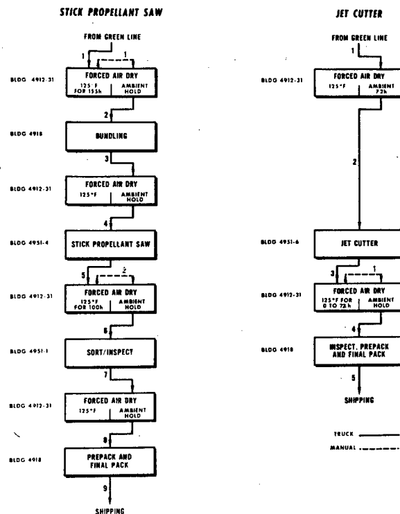
Figure 2 - Transportation Steps of Benite Processing
