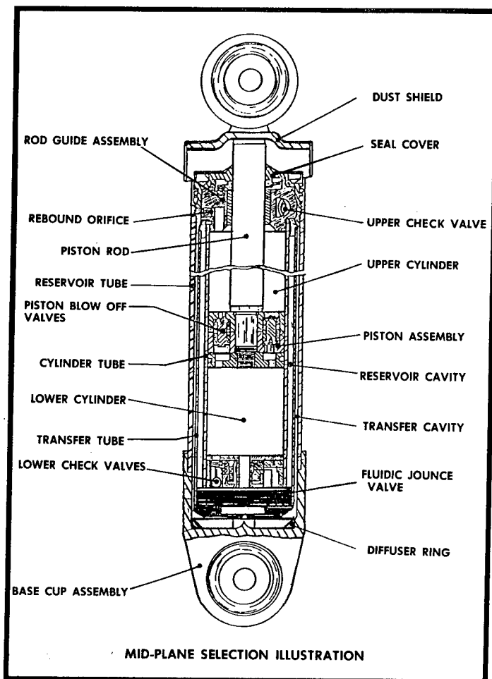
Figure 1 - Fluidic Damper
