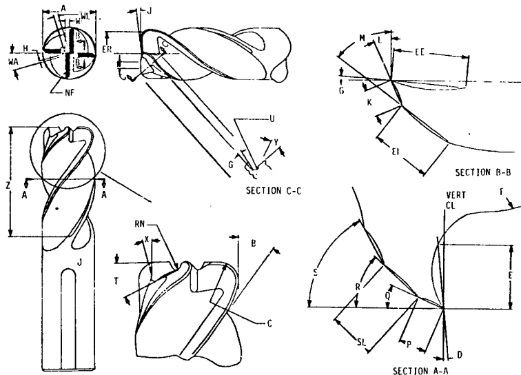
Figure 2 - Cutter Geometry
