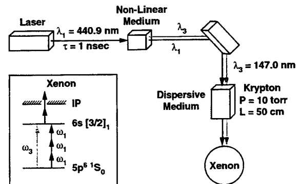
FIG. 1. Standard (3+1)-photon phase-control experiment. A fundamental field from a laser is tripled in a nonlinear medium and then both the fundamental and third harmonic pass through a dispersive medium. Since the refractive indices of the dispersive medium for the fundamental and third-harmonic fields are different, a relative phase difference between the two fields is created. Our numerical simulations consider (3+1)-photon phase control of xenon photoionization, where IP stands for ionization potential.
