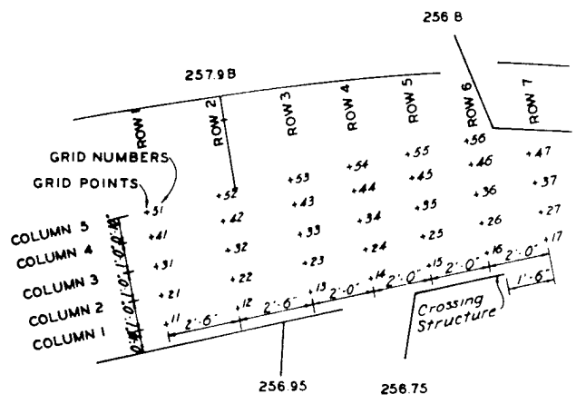
GRID LAYOUT FOR DEPTH INDICATORS FIGURE 9
