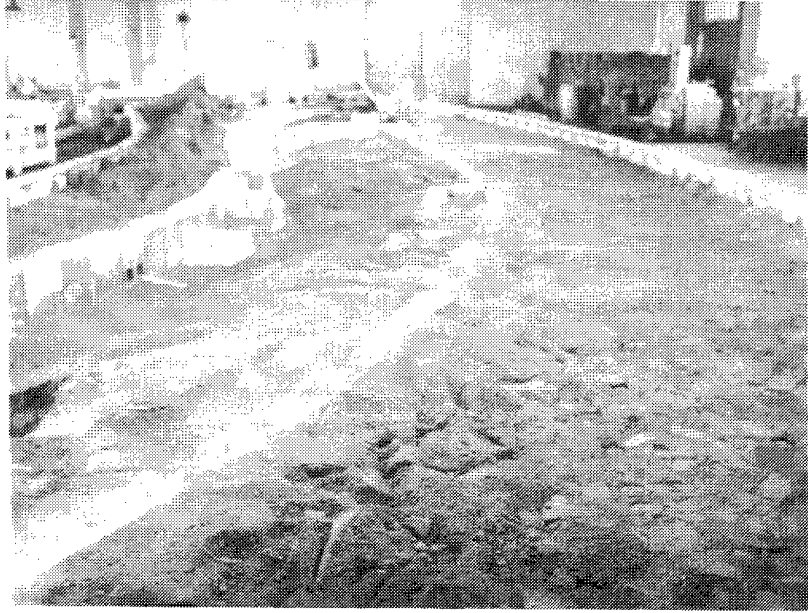
5 View upstream from about RM 245 during process of back-filling channel and bank areas with ground walnut shells.
