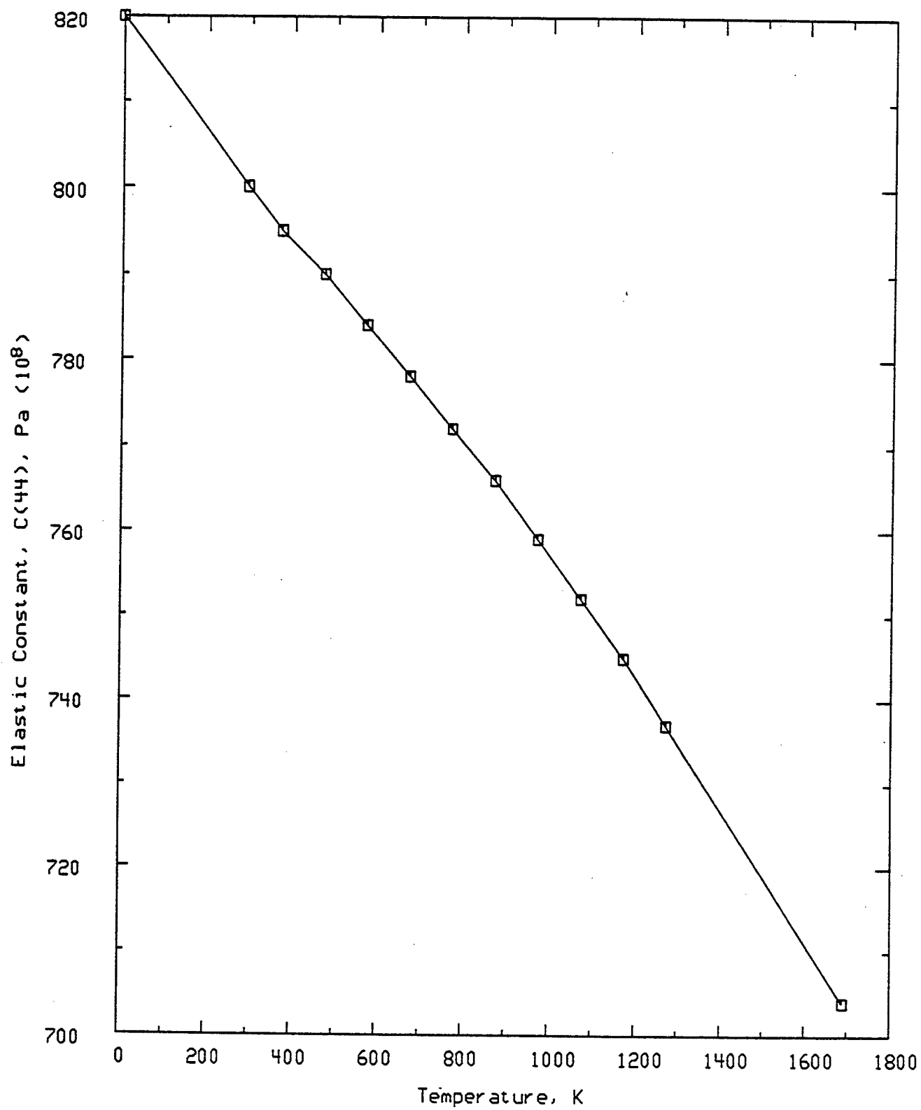
Figure 110 Elastic Constant, C(44) of Silicon, p-type
