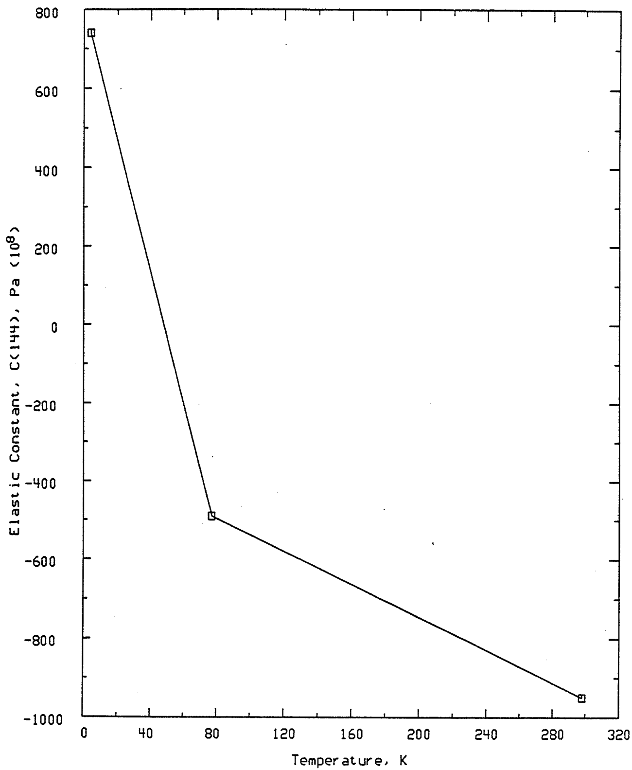
Figure 118 Elastic Constant, C_{\langle 144 \rangle} of Silicon
