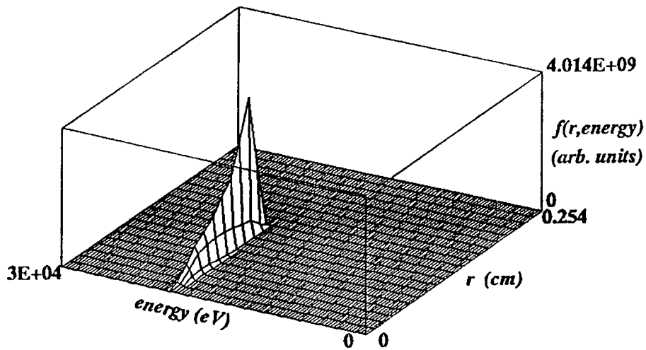
Figure 5.6: Kinetic energy distribution at the beam exit plane, z = 8 \text{ cm} .
