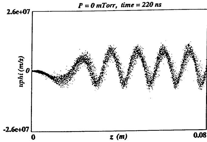
Figure 5.5: Azimuthal velocity as a function of axial position. Note that \langle u\phi \rangle = \langle v\phi \rangle = \langle r\dot{\phi} \rangle > 0 , resulting in a slight net focusing of the beam.
