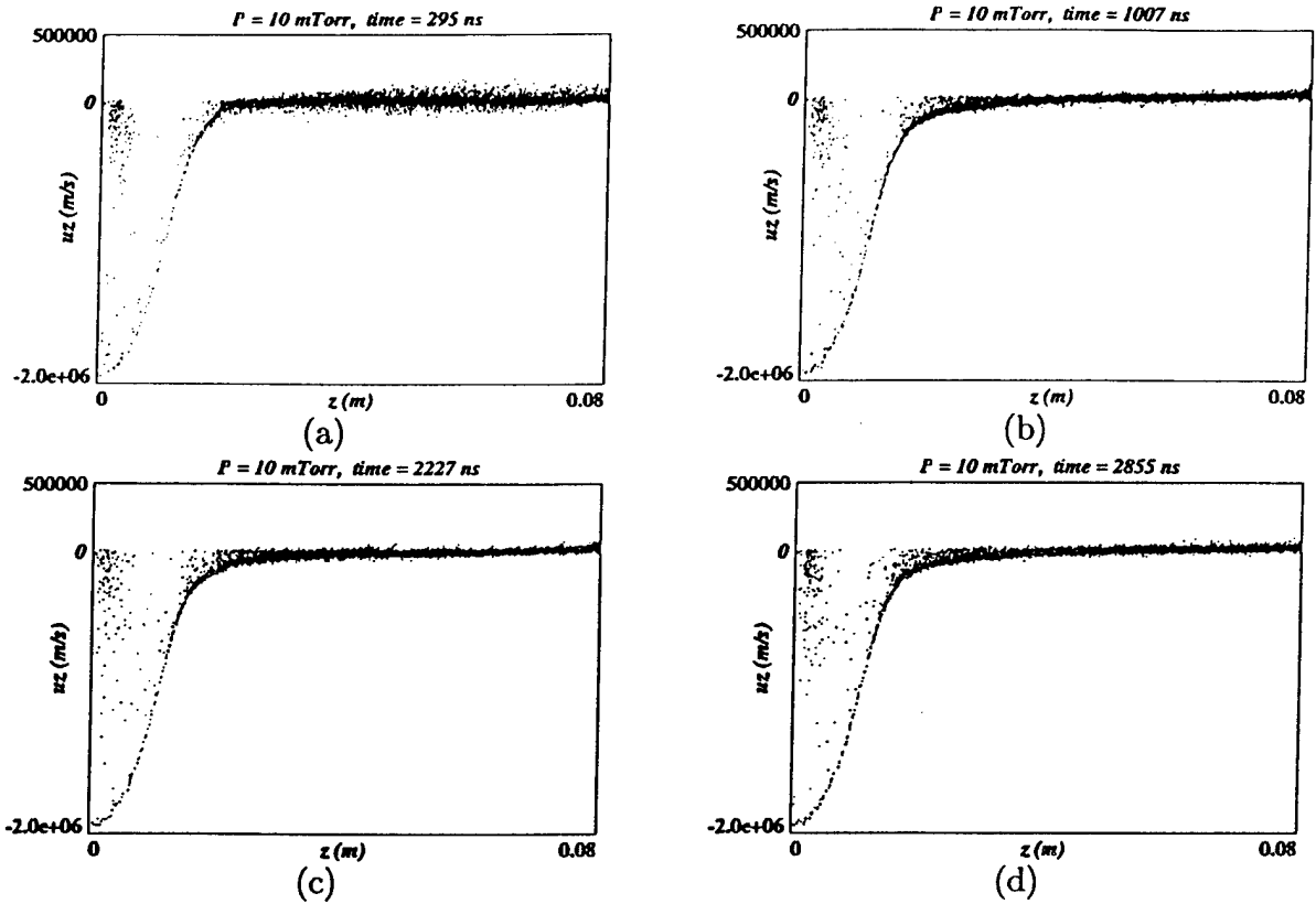
Figure 5.36: Axial velocity component of hydrogen ions for a series of times.
