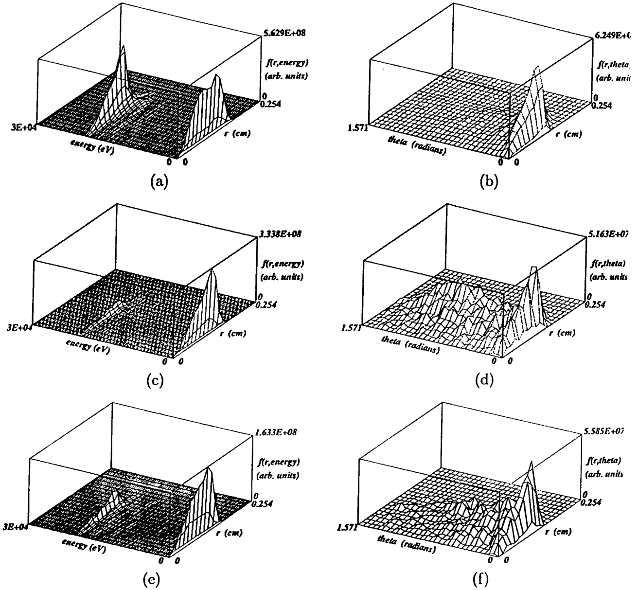
Figure 5.46: Energy distribution functions and exit angle of velocity vector with respect to the normal of ionization electrons at the beam exit for a series of times, (a,b) 295 ns, (c,d) 1738 ns, and (e,f) 2227 ns. The gas pressure was 10 mTorr.
