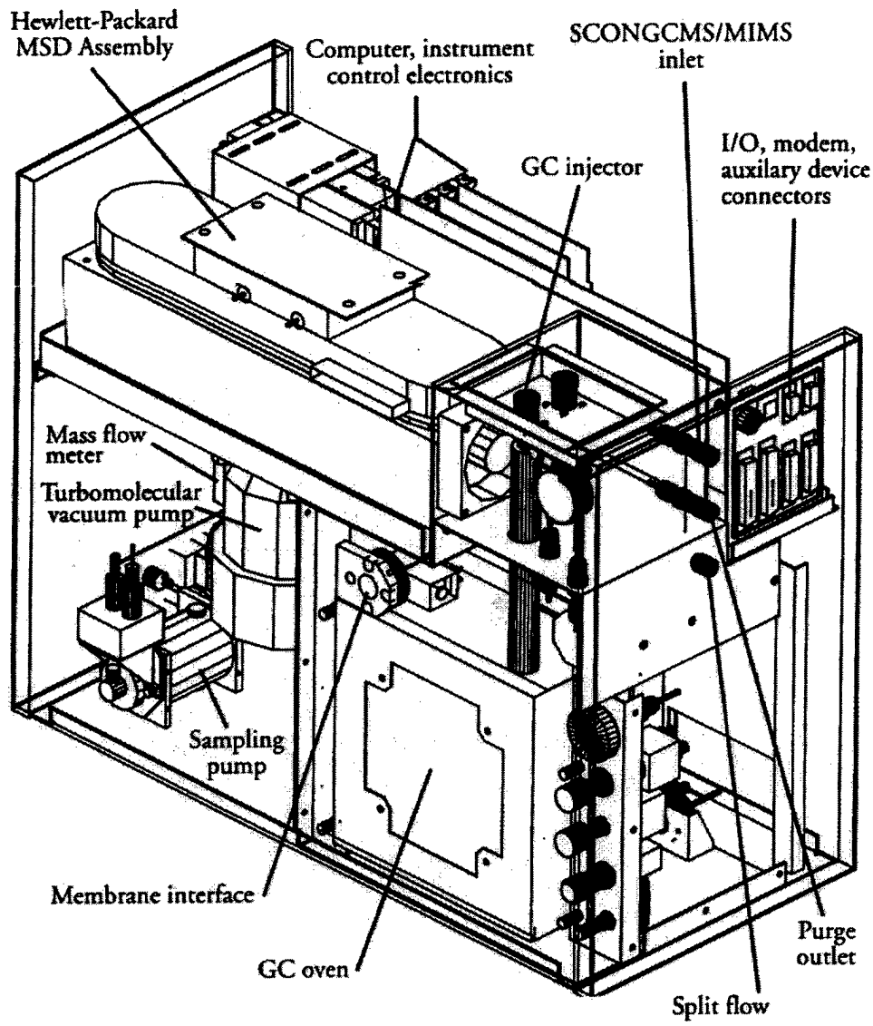
Figure 8-1. A breakaway view of the Viking SpectraTrak™ 572 Portable GC/MS. (Courtesy of Viking Instruments.)
