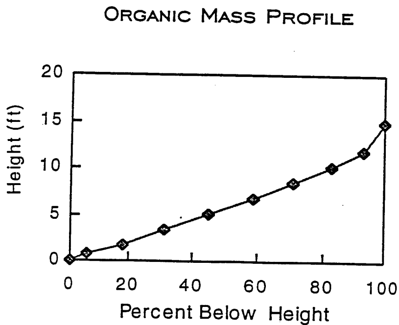
Figure 12. Cumulative Distribution of Metal and Organic Constituents at Various Heights Across the Exhaust Face for Booth 1, (to ensure conservative results, one outlying data point was omitted from the average results obtained to derive the metals graph).
