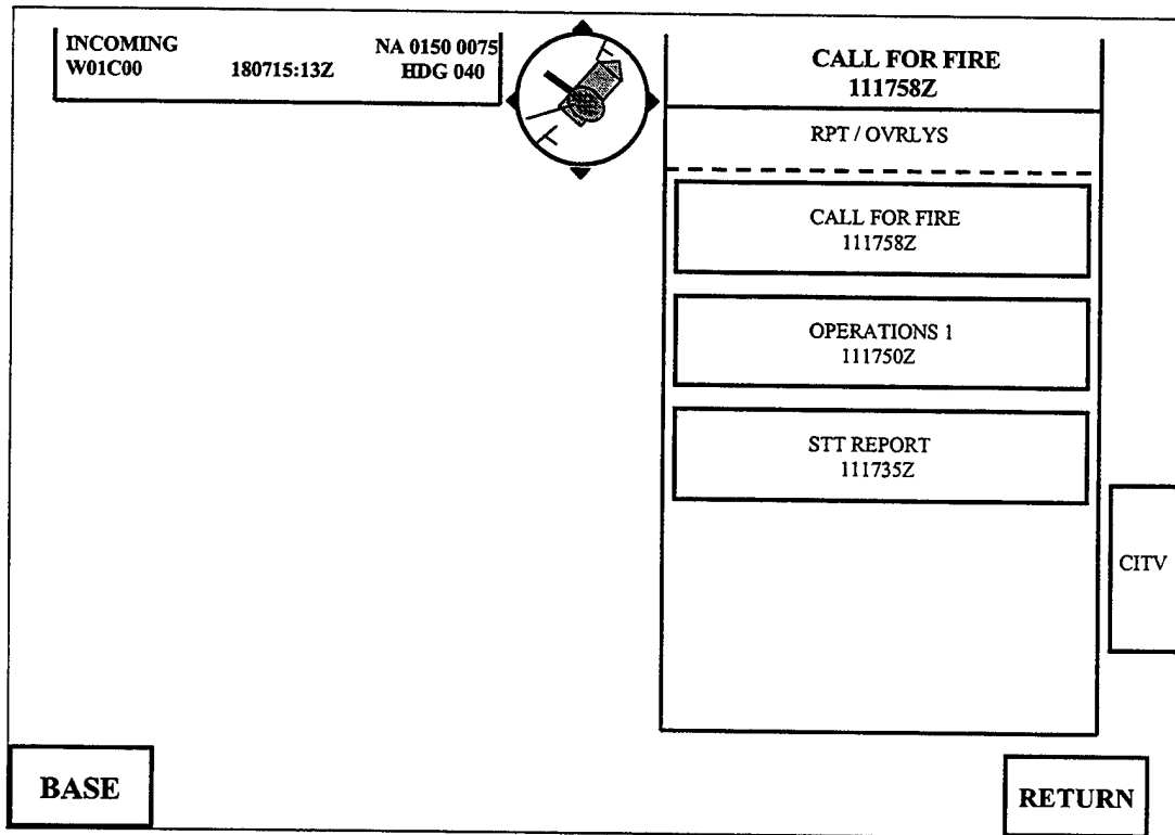
Figure 5. Incoming Message Screen
