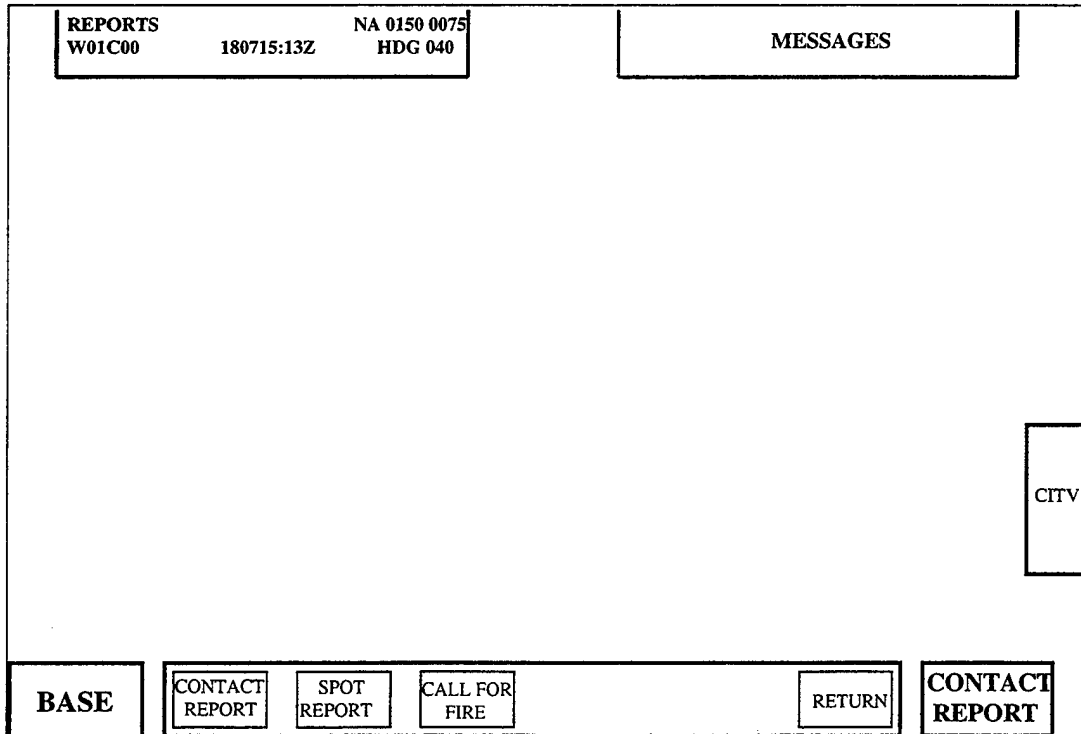
Figure 7. Report Screen
