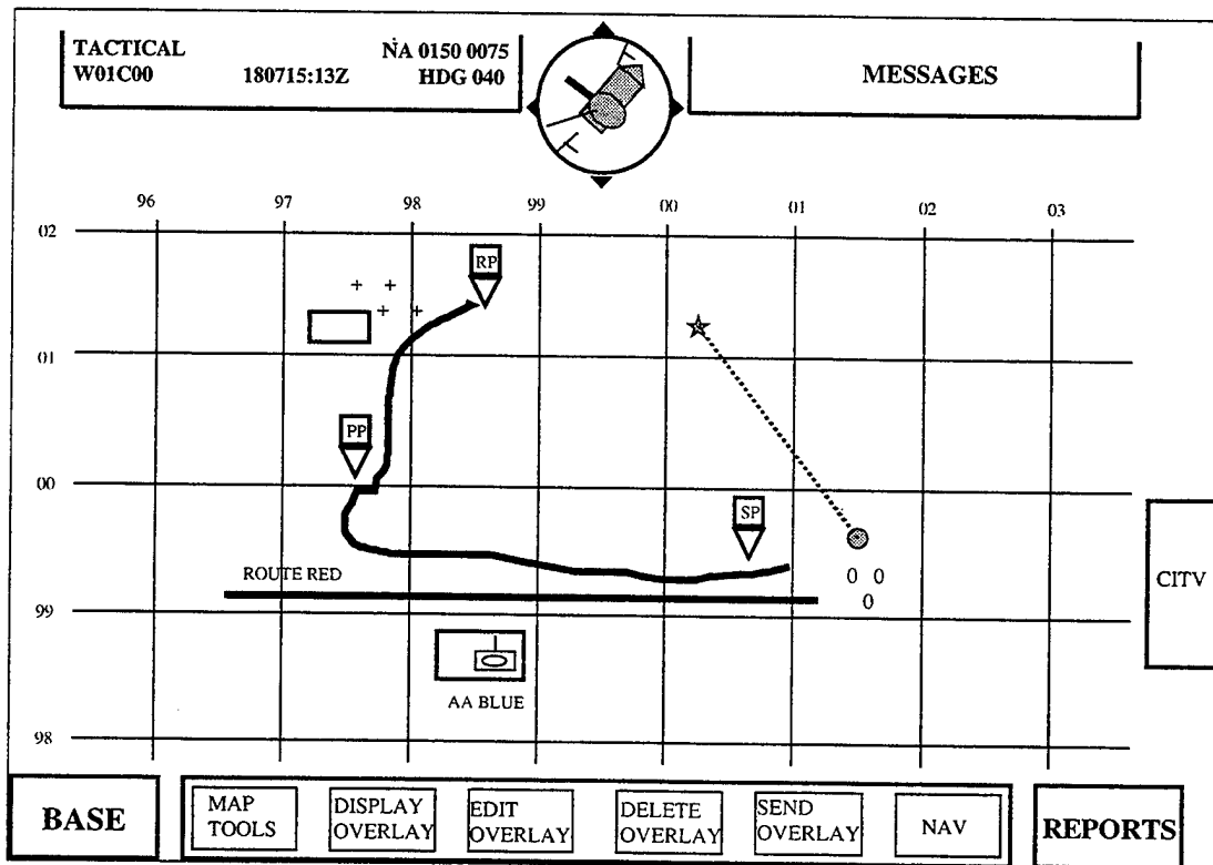
Figure 3. Tactical Screen
