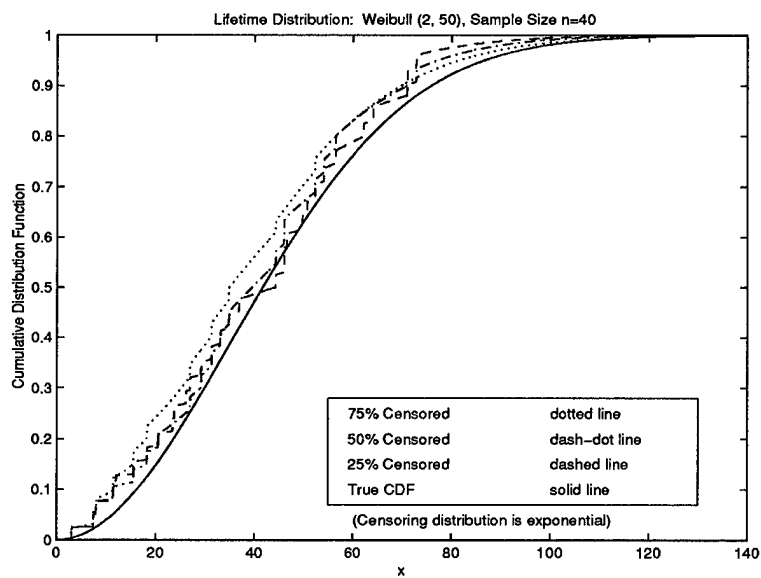
Figure 38 Klein, Lee, and Moeschberger Estimator, Weibull with shape 2.
