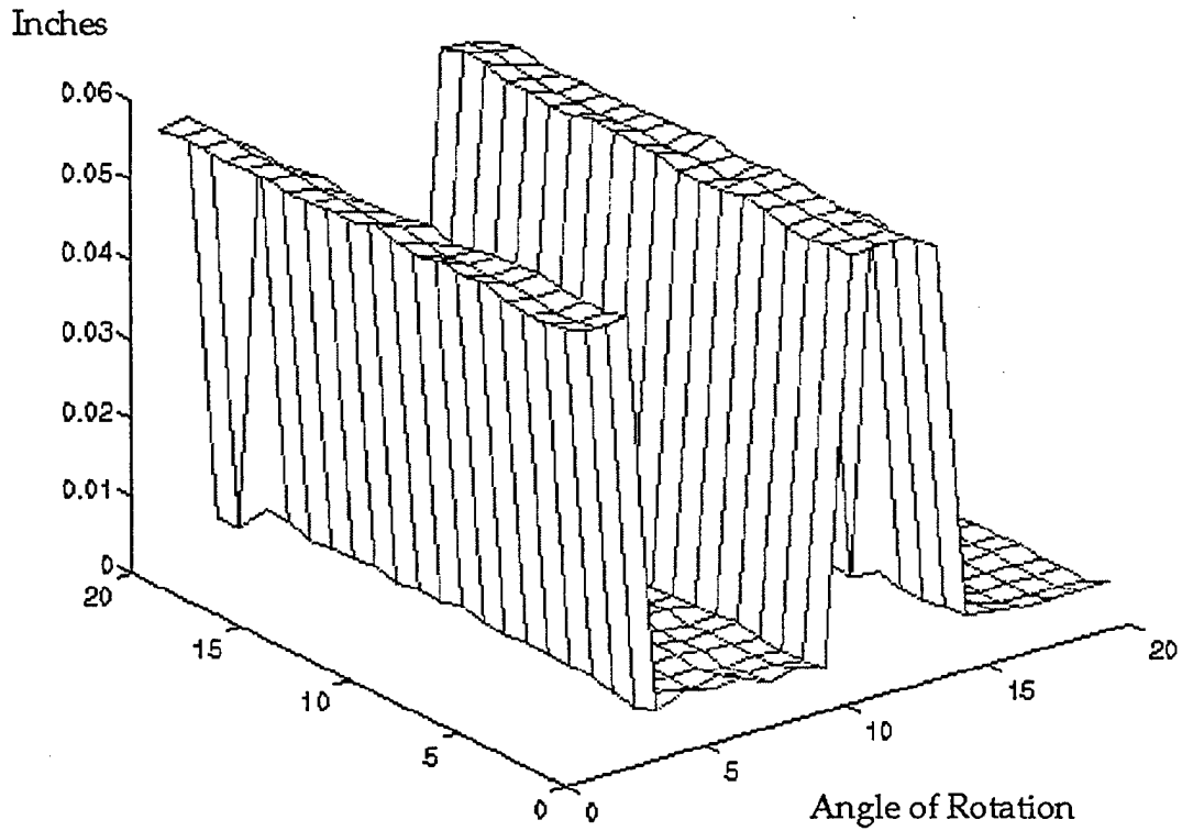
Figure 7. Lands and grooves from an uneroded tube.
