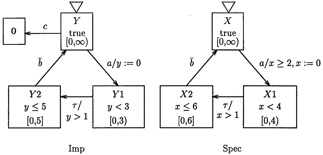
Figure 6. Simple Y \circ \xrightarrow{\delta}_i X TSA.
