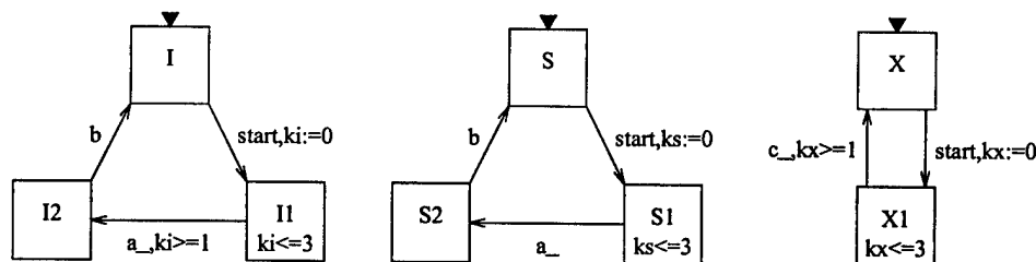
Figure 7. I \circ_{\leq i} S \not\Rightarrow I \parallel X \circ_{\leq i} S \parallel X .
