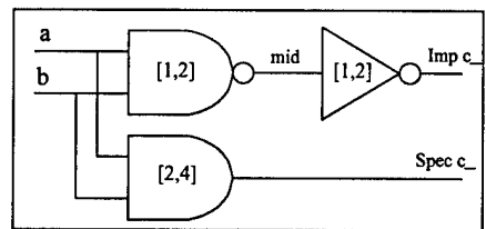
Figure 22. And Implementation and Specification in Parallel.
