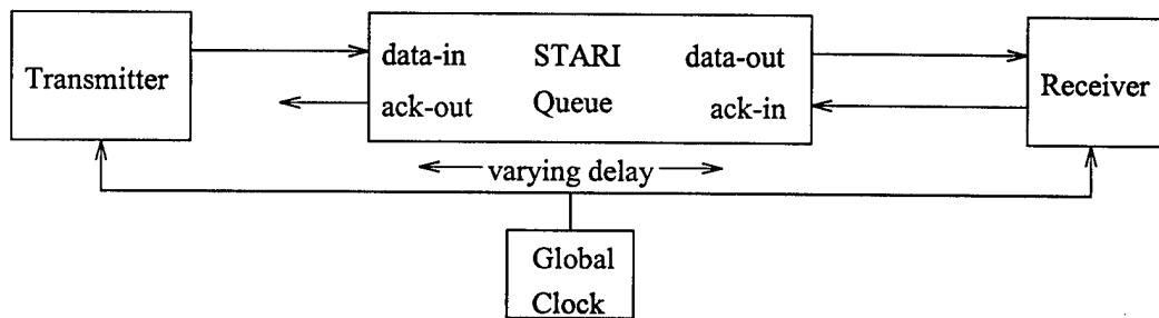
Figure 29. STARI Environment.
