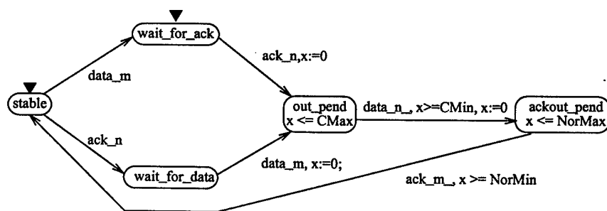
Figure 27. Abstract STARI FIFO Queue Stage Timed Process.
