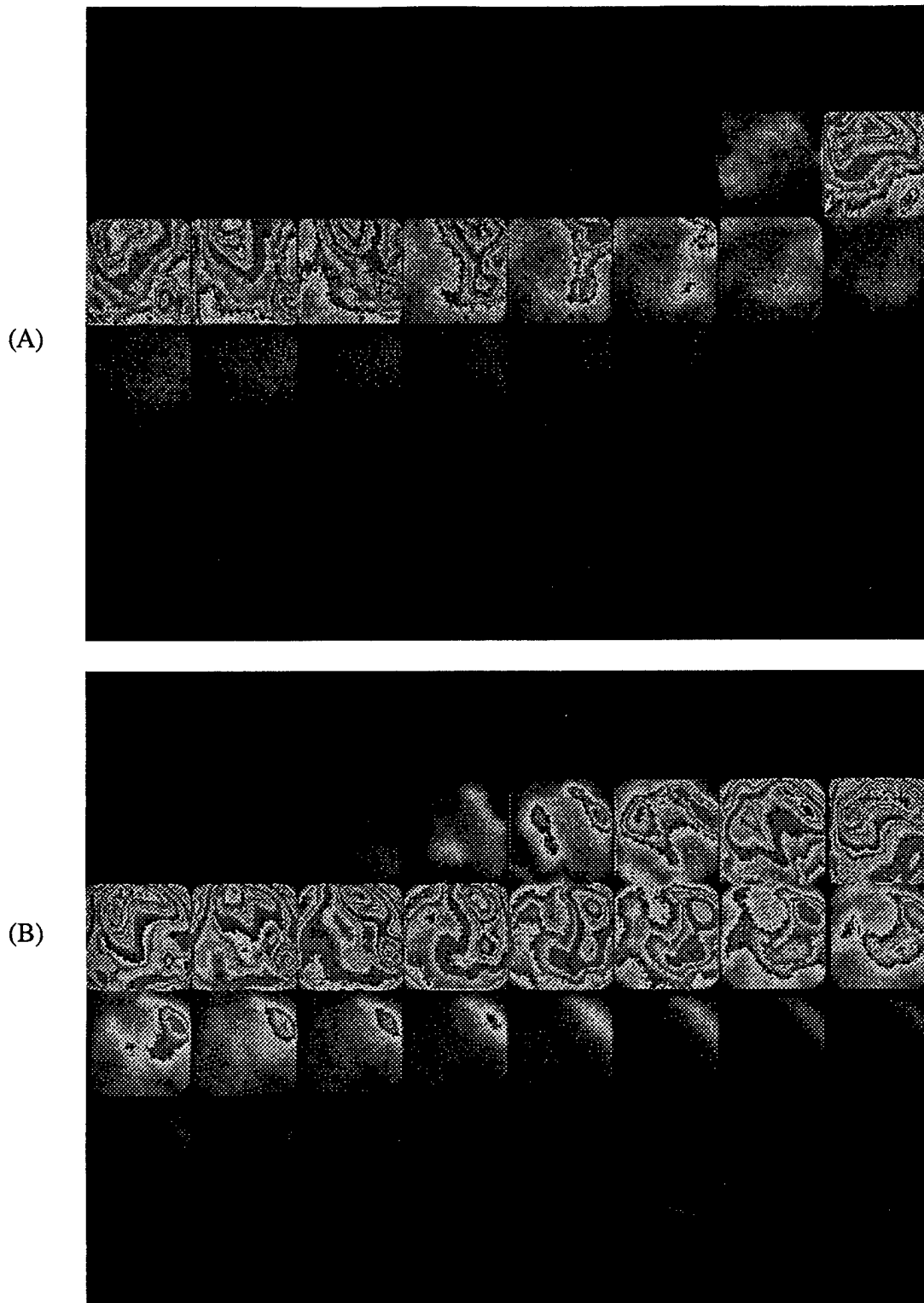
Fig. 10. High-speed Spectral Images with intake air at 38°C, an overall air/fuel ratio of 30-1 and injection pressure of 30,625 psi (210 Mpa): (A) 2.47 \mu m and (B) 3.42 \mu m.
