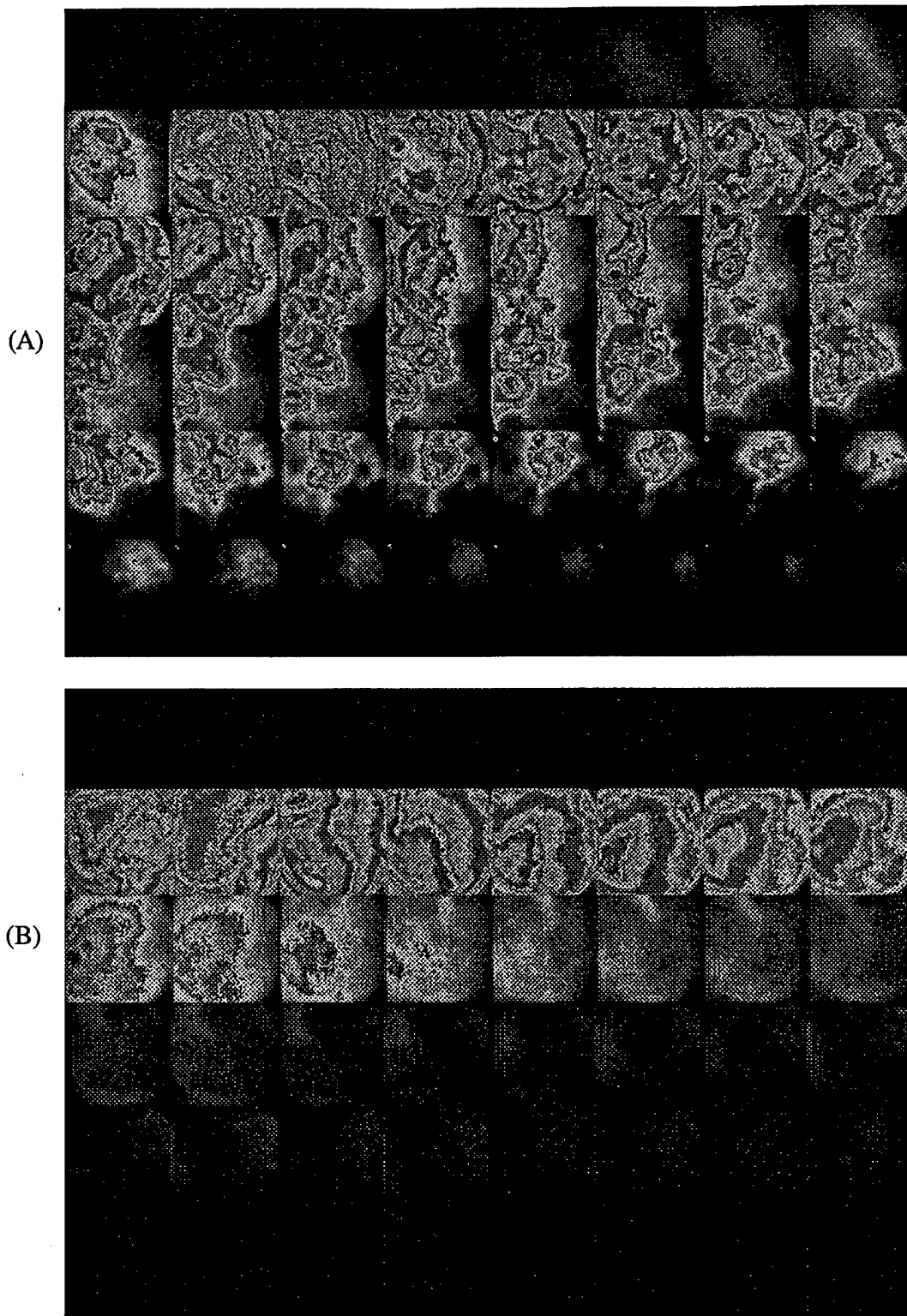
Fig. 7. High-speed Spectral Images from DI-CI engine with an overall air/fuel ratio of 22.7 and injection pressure of 25,375 psi (175 Mpa): (A) 3.8 \mu m and (B) 2.2 \mu m.
