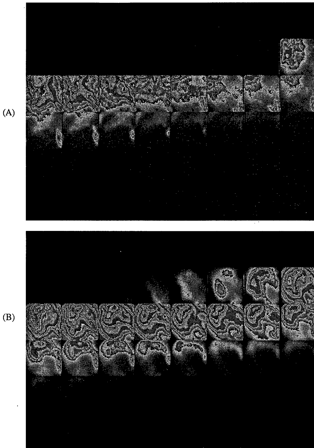
Fig. 8. High-speed Spectral Images with intake air at 38°C, an overall air/fuel ratio of 30-1 and injection pressure of 16,625 psi (114 Mpa): (A) 2.47 \mu m and (B) 3.42 \mu m.
