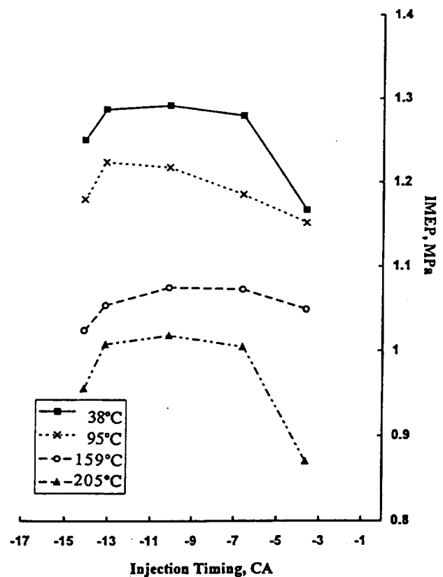
Fig. 4. IMEP for Varied Injection Timing and Intake Air Temperature (1000rpm, Rail Pressure 12Mpa).
