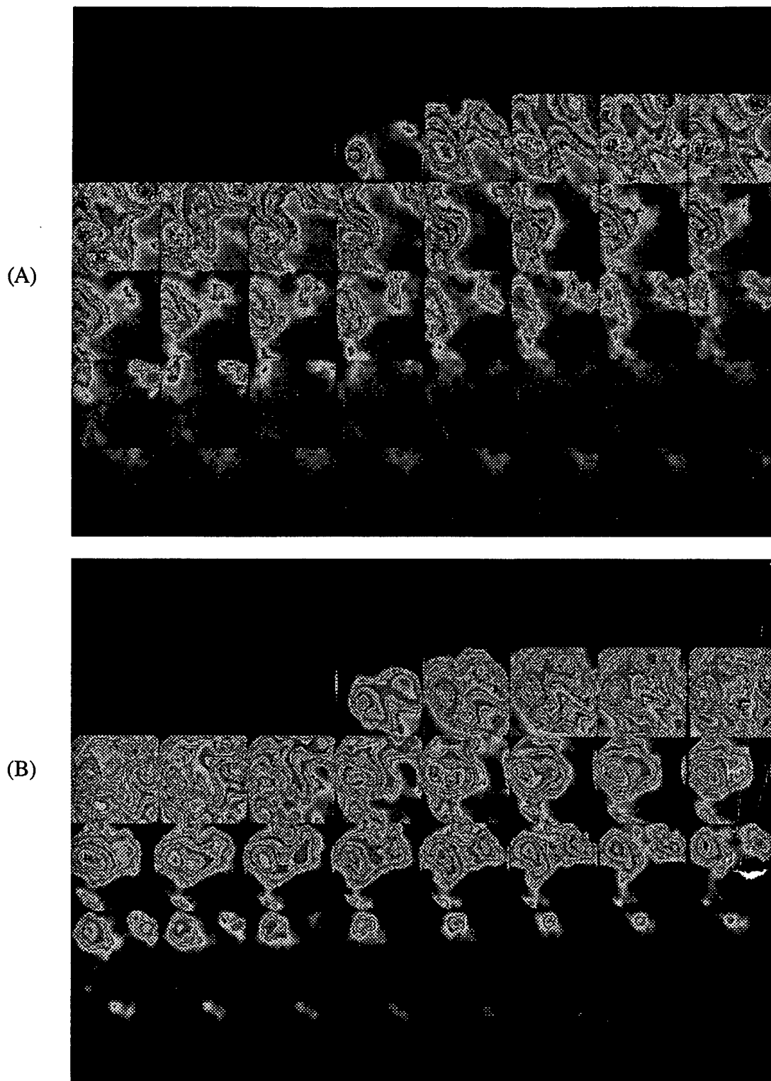
Fig. 9. High-speed Spectral Images with intake air at 150°C, an overall air/fuel ratio of 30-1 and injection pressure of 16,625 psi (114 Mpa): (A) 2.47 \mu\text{m} and (B) 3.42 \mu\text{m} .
