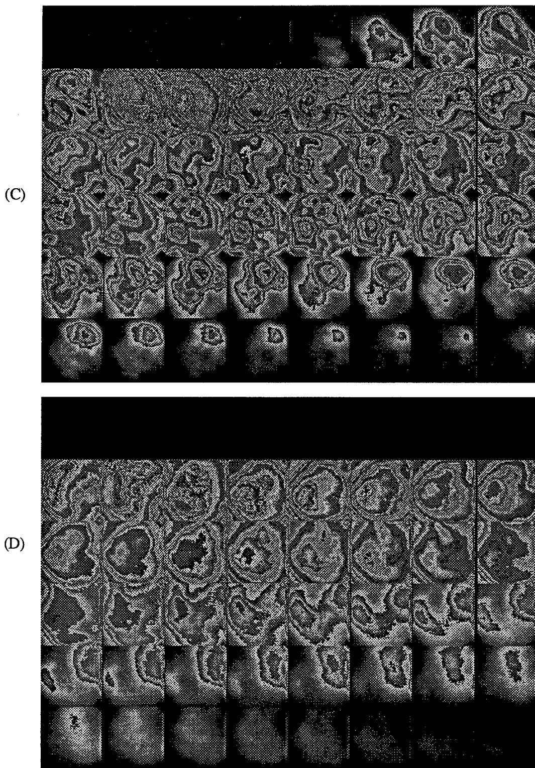
Fig. 7. High-speed Spectral Images from DI-CI engine with an overall air/fuel ratio of 22.7 and injection pressure of 25,375 psi (175 Mpa): (C) 3.42 \mu m and (D) 2.27 \mu m.
