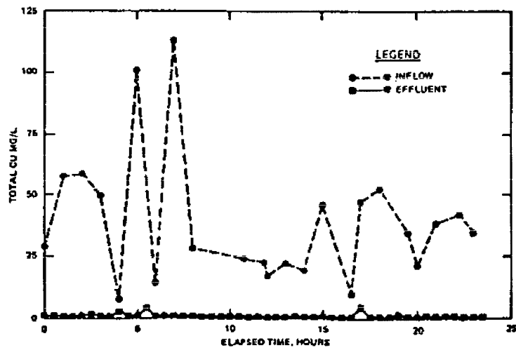
Figure 22. Influent and effluent copper concentrations
