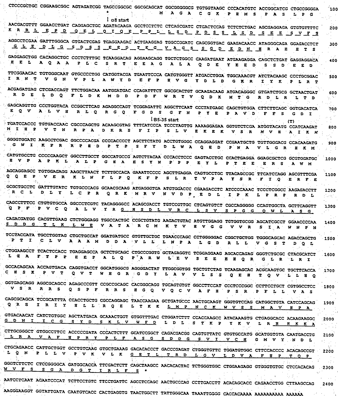
Figure 8 Nucleotide and deduced amino acid-sequences of the bop1 cDNA. The full-length bop1 cDNA encodes a protein of 732 amino acids containing four WD40 repeats (underlined). The PEST sequence in the amino-terminus is underscored by a dash line. The starting positions of clones B5-35 and x8 are indicated by arrows. The two ATG codons at the start of the B5-35 open reading frame are at nt 781 and 799. (T) denotes a single-base substitution found in B5-35 when compared to the sequence of clone a8 isolated from the cDNA library. Asterisks indicate in-frame stop codons
