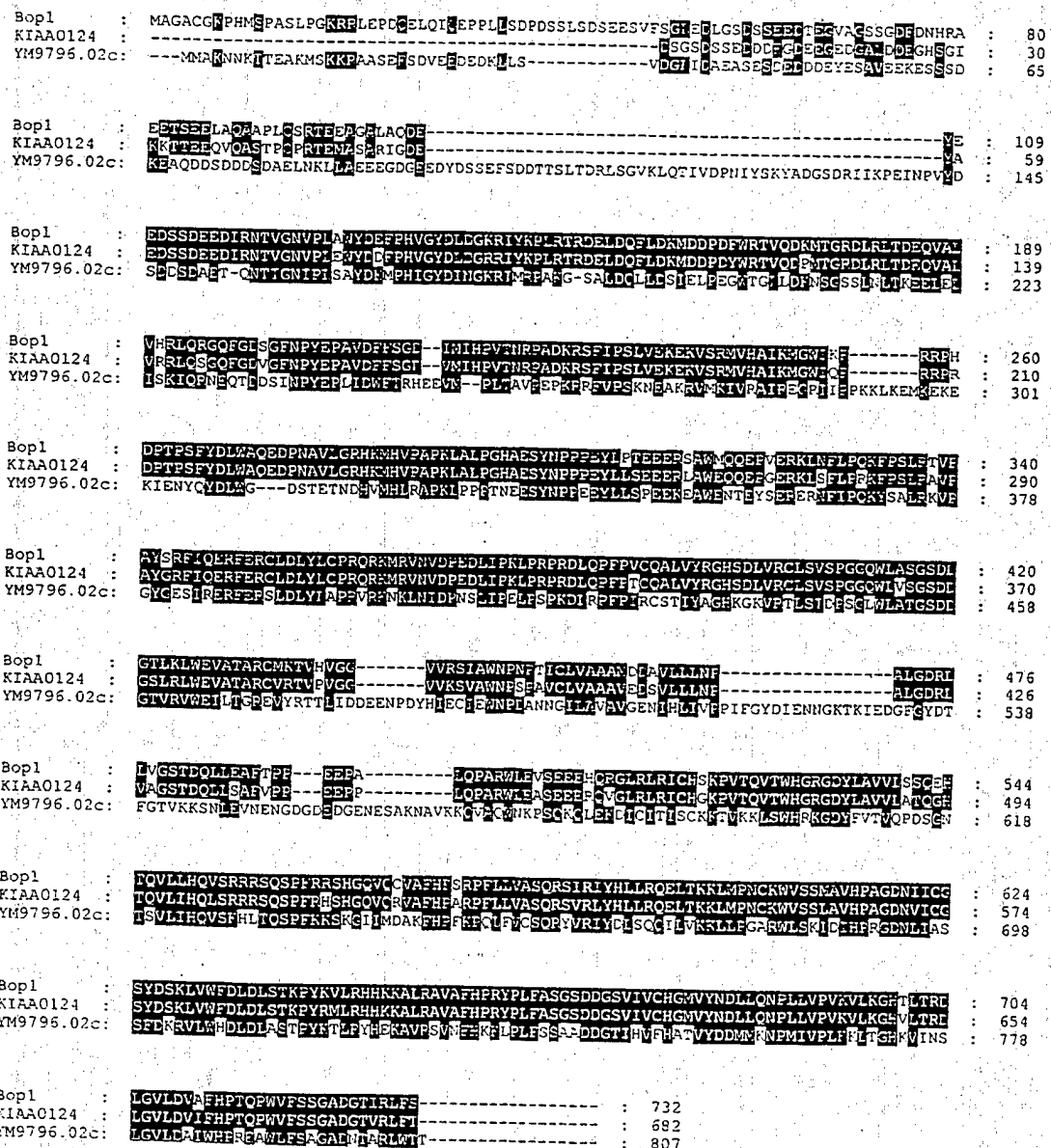
Figure 9 Comparison of amino acid sequences of the murine Bop1 and its human (KIAA0124) and yeast (YM9796.02c) homologs. Alignment was compiled using the Clustal W program (Thompson et al., 1994) and modified by using GeneDoc (Nicholas et al., 1997). Shading indicates identical positions and conservative substitutions
