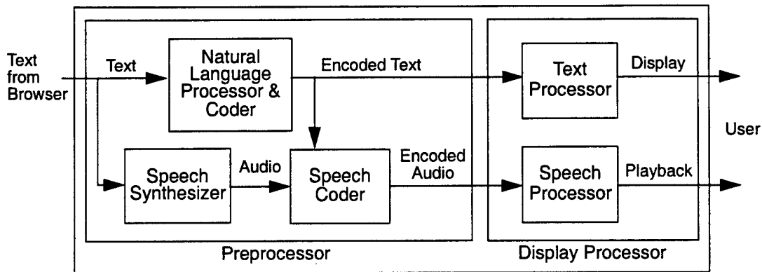
Figure 6. Text-Only Architecture
