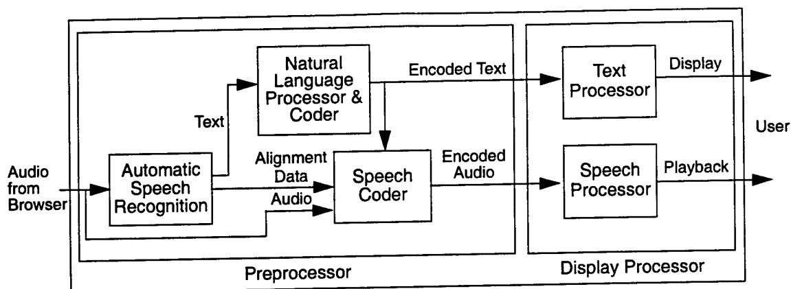
Figure 7. Audio-Only Architecture
