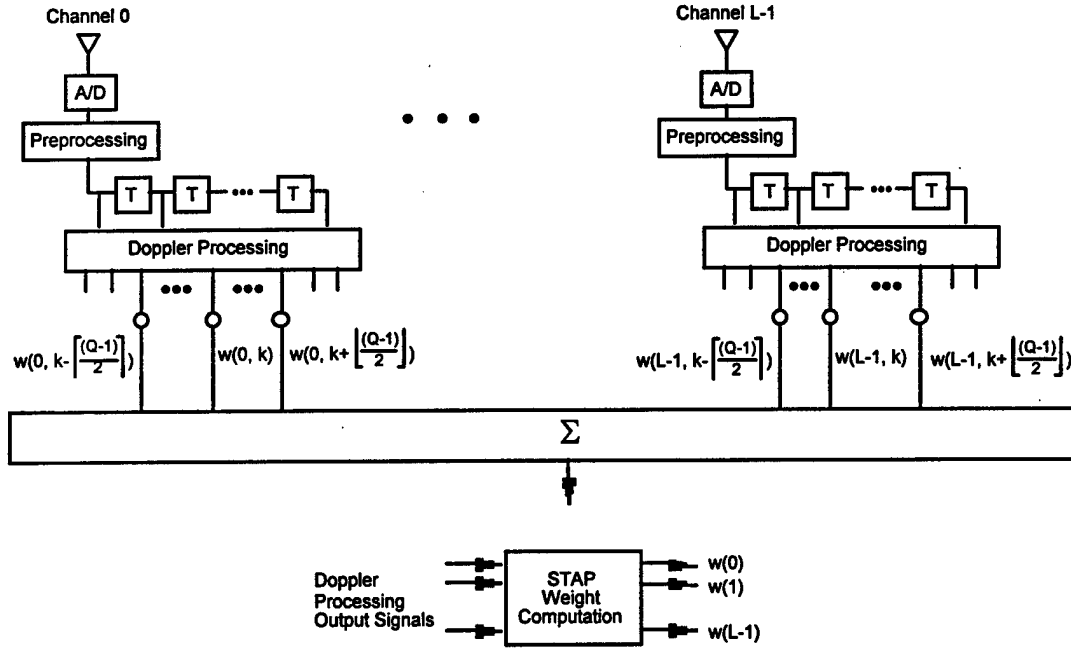
Figure C.4 – High-order Doppler-factored STAP.
