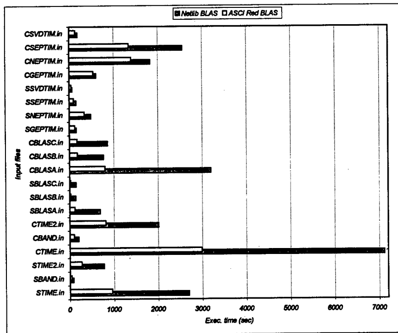
Figure 17 – Performance showed in the timing routines for two different versions of LAPACK.
