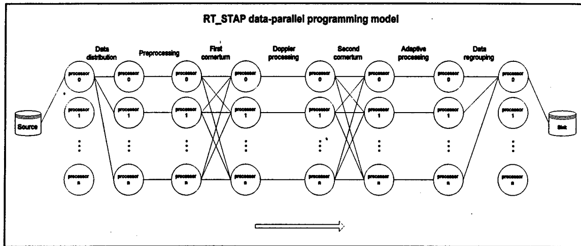
Figure C.1 – Graphical representation of RT-STAP parallel implementation.
