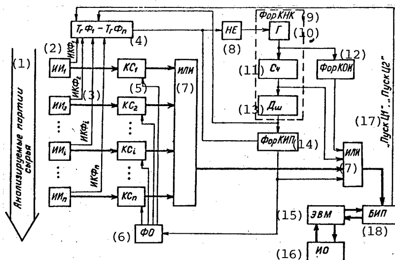
Figure 2. Functional structure of switching unit.
