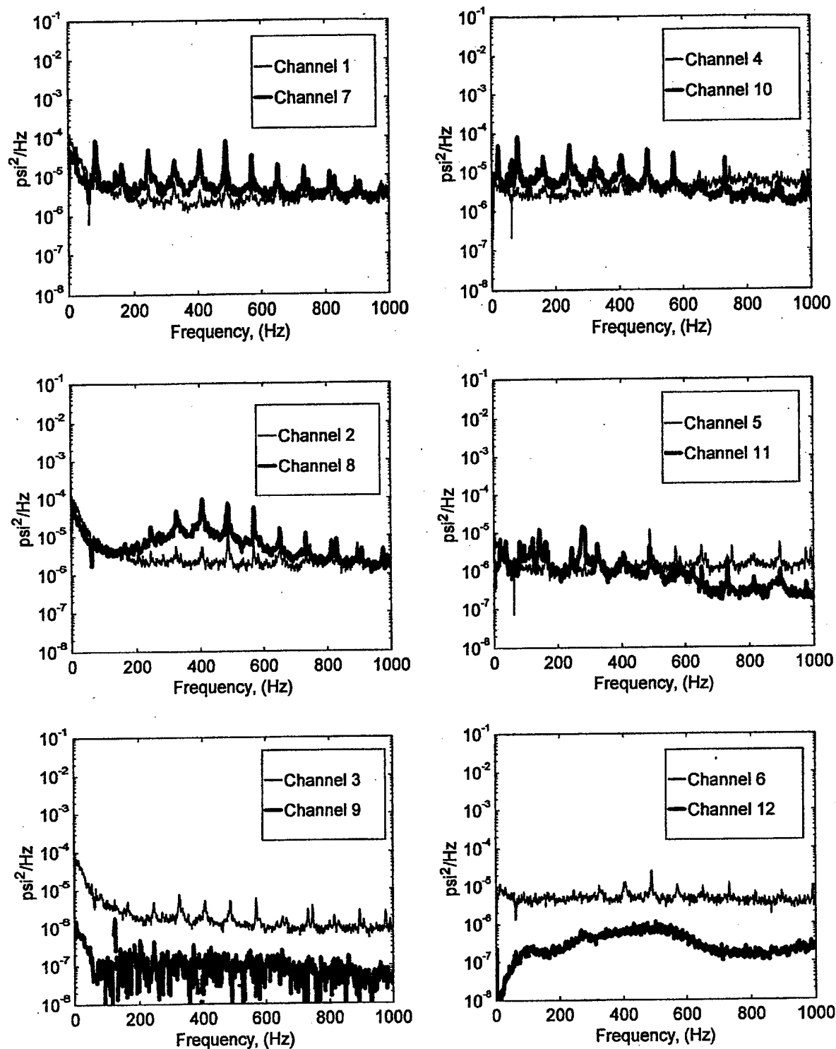
FIGURE B-16. PRESSURE POWER SPECTRAL DENSITY (RUN 7, POINT 4) (\bar{q} = 45 \text{ psf}, \alpha = 10^\circ, \psi = 0^\circ)
