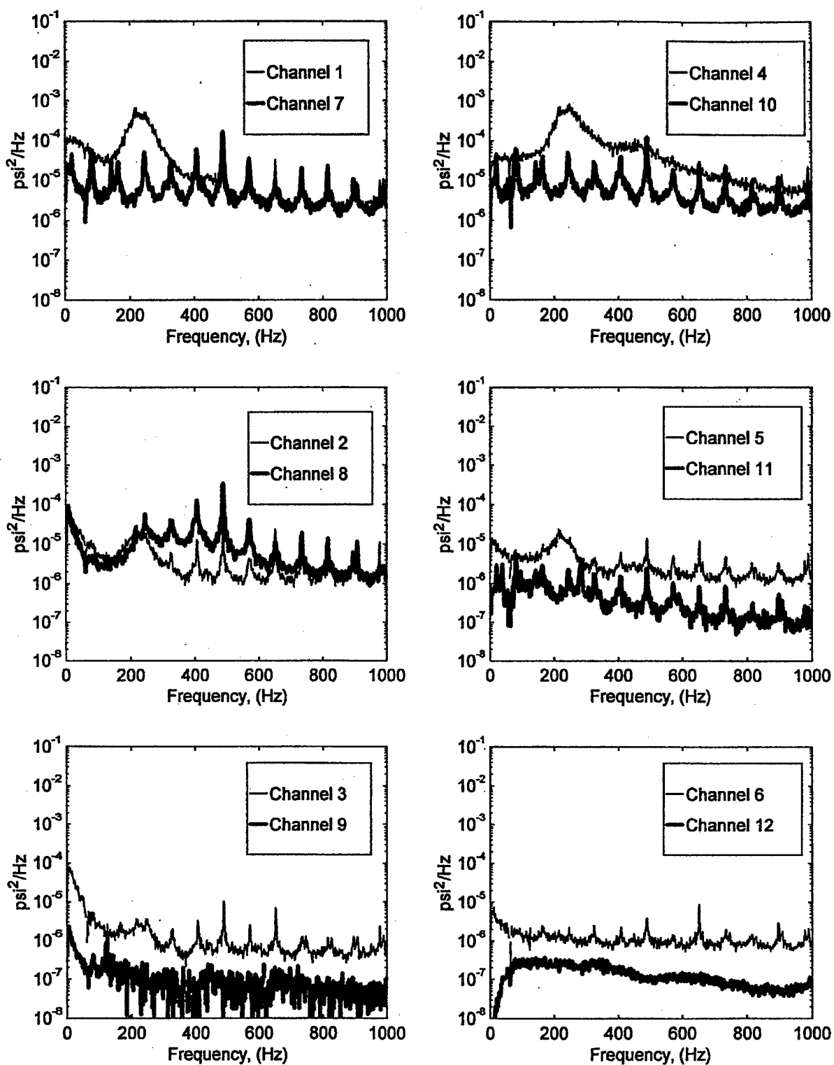
FIGURE B-27. PRESSURE POWER SPECTRAL DENSITY (RUN 9, POINT 3)
