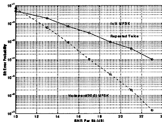
Figure 1. BER performance of Hadamard (20,5) MFSK and 1-of-4 MFSK with diversity 2 (D2) selectable and is optimally set to the length of time significant multipath persists in the communication channel. Clearly this
