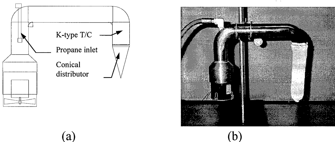
Figure 4 Gas Train Prototype (a) schematic and (b) assembly under test with ytterbium oxide mantle
