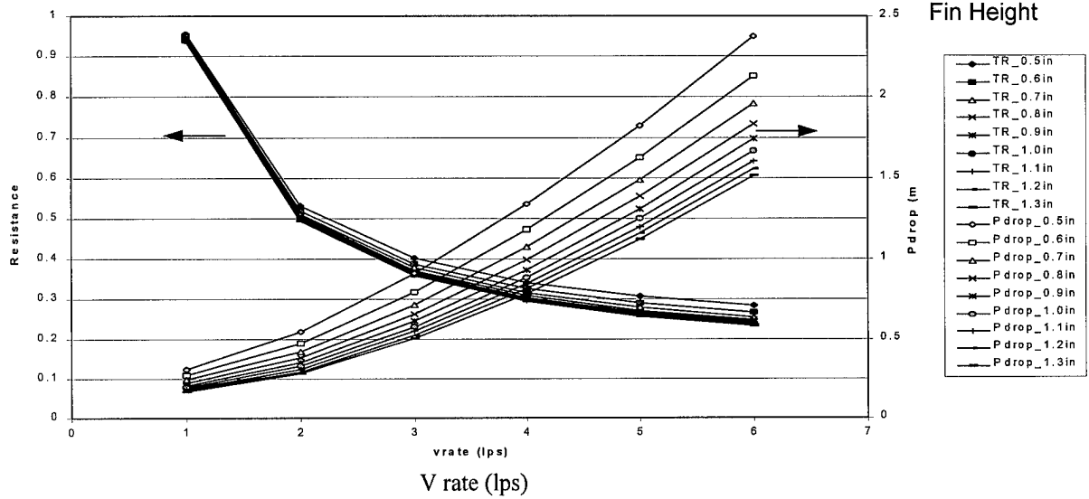
Graph 2: Thermal Resistance and Pressure Drop vs. Flow Rate for a fin pitch of 20 fins/inch
