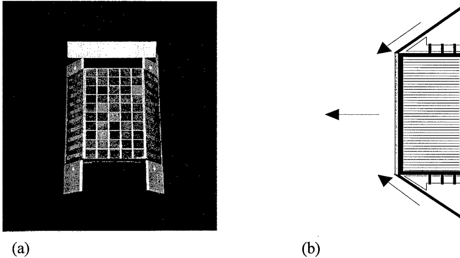
Figure 27. (a) Photo of hexagonal photovoltaic array assembly showing thin brackets for support (b) bending forces acting on array while heat exchanger fixed in position by screws.
