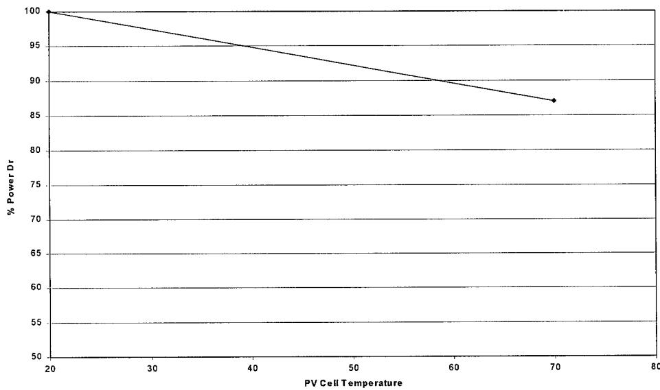
Graph 3: Percentage Performance Drop in Power Output of Ammonix Cells
