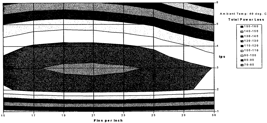
Graph 5: Minimization of Power Loss Fin Height 0.75 in.
