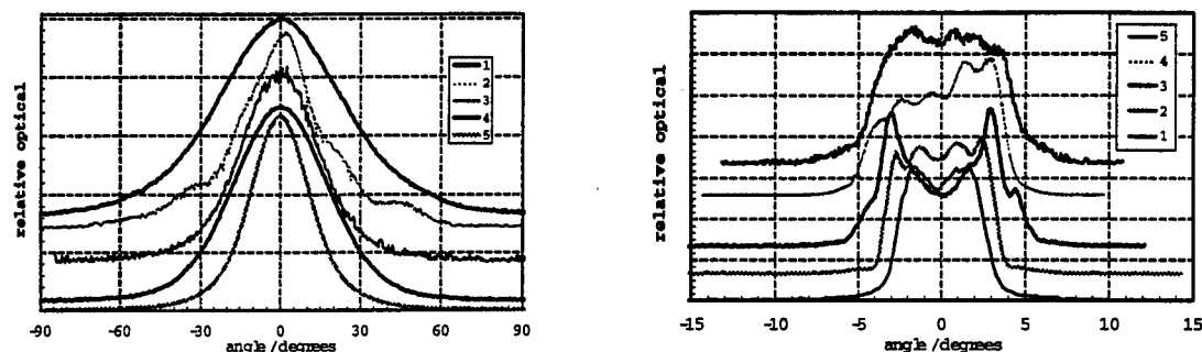
Fig. 7 Angular distributions of the fast axis emission (a) and for the slow axis (b) for different types of high power diode laser bars.
