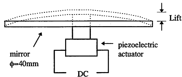
Figure 9. Sketch of the adaptive mirror
