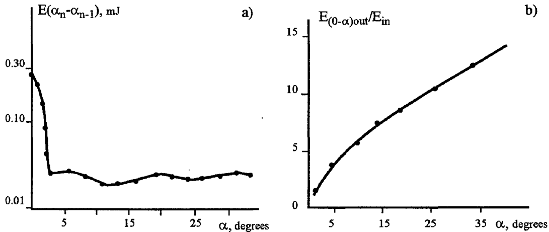
Fig. 7. Measurement results for scattered radiation.
