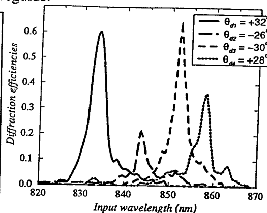
Fig. 4: Diffraction spectra of the 4-channel WDM.
